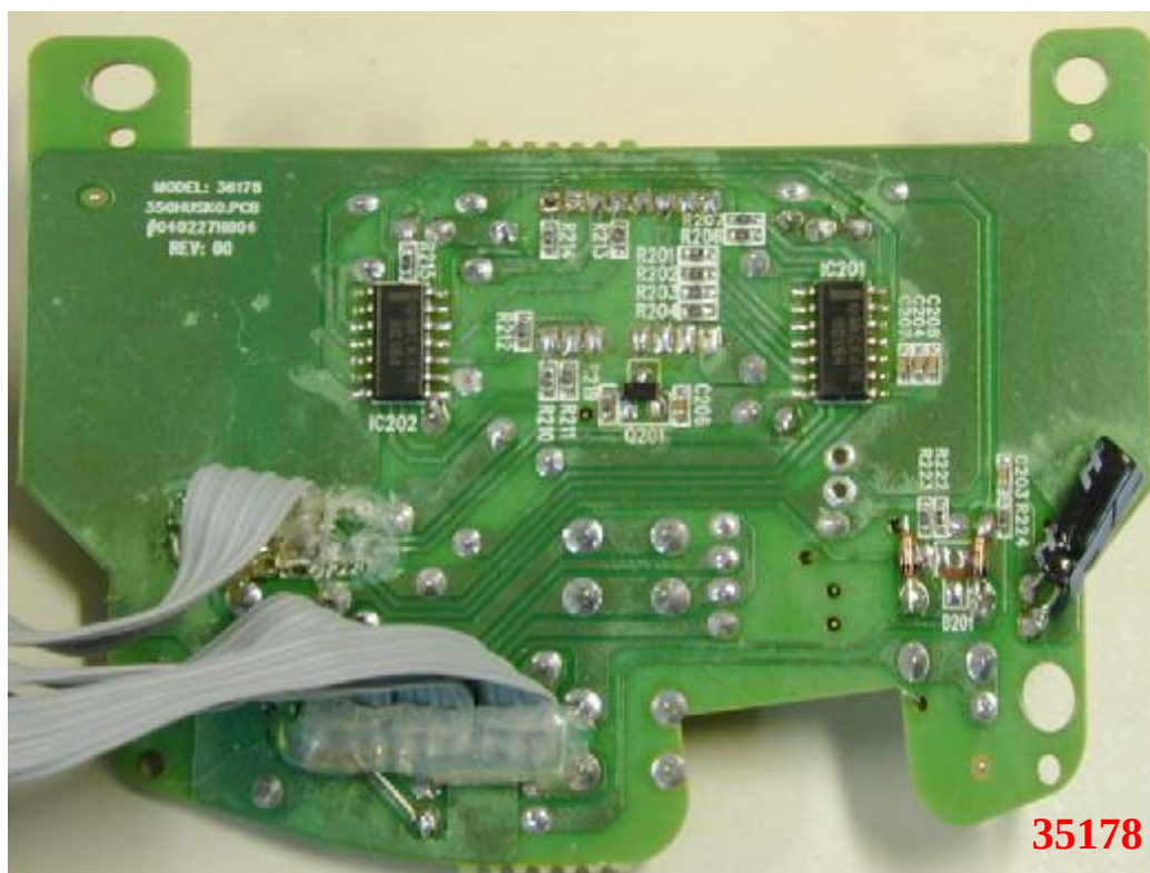
Photo 6: Internal photo of EUT (Base)
