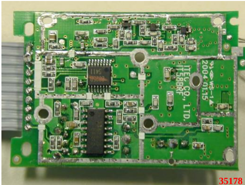
Photo 15: Internal photo of EUT (Base)
