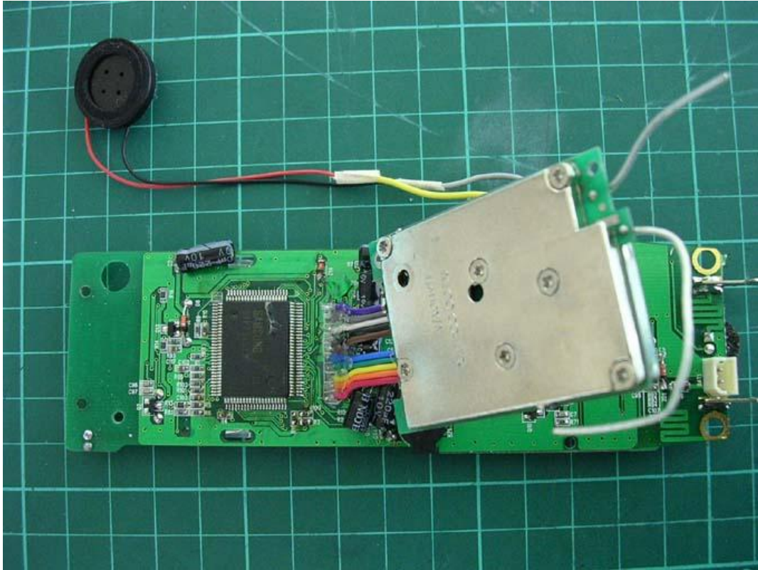
Photo 2: Internal photo of EUT (Handset)
