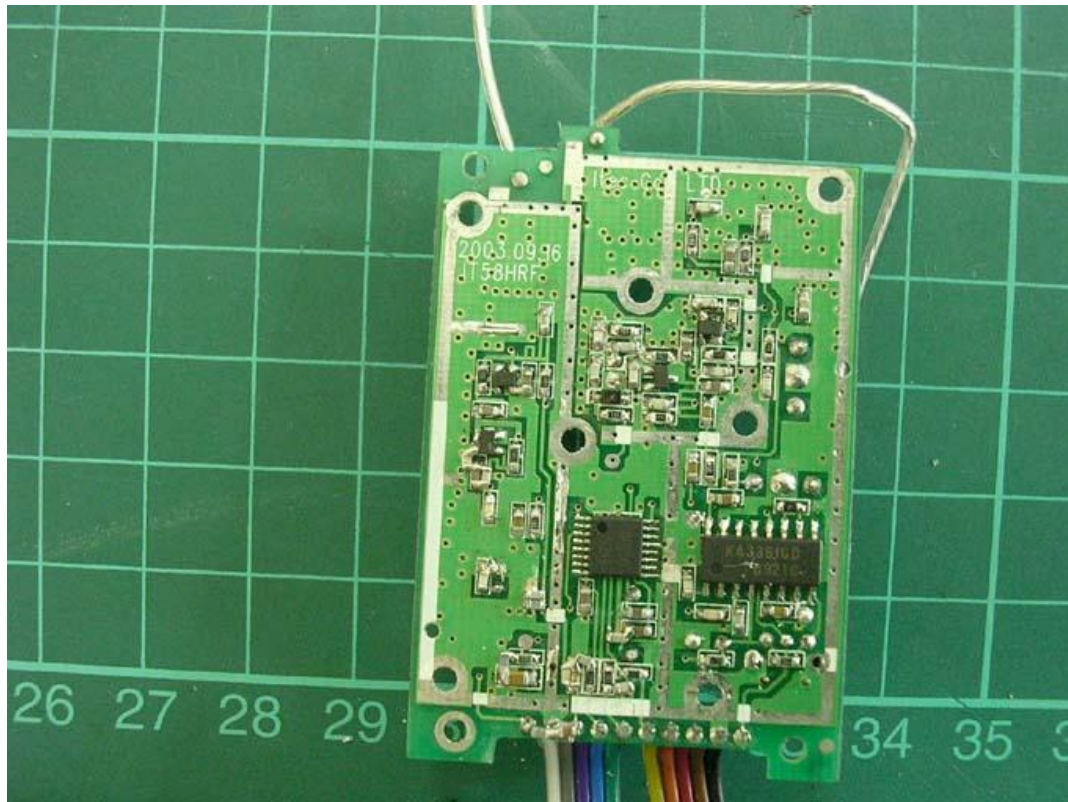
Photo 5: Internal photo of EUT (Handset)
