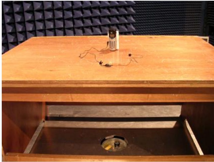
Photo 3: Radiated Emission Test Set-up (Handset)
