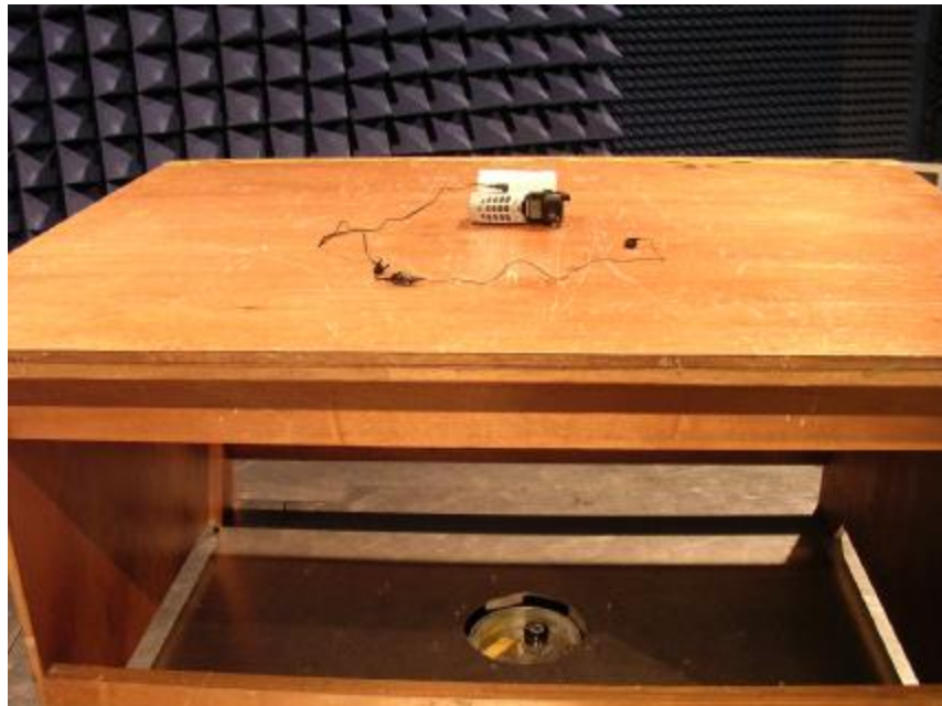
Photo 2: Radiated Emission Test Set-up (Handset)
