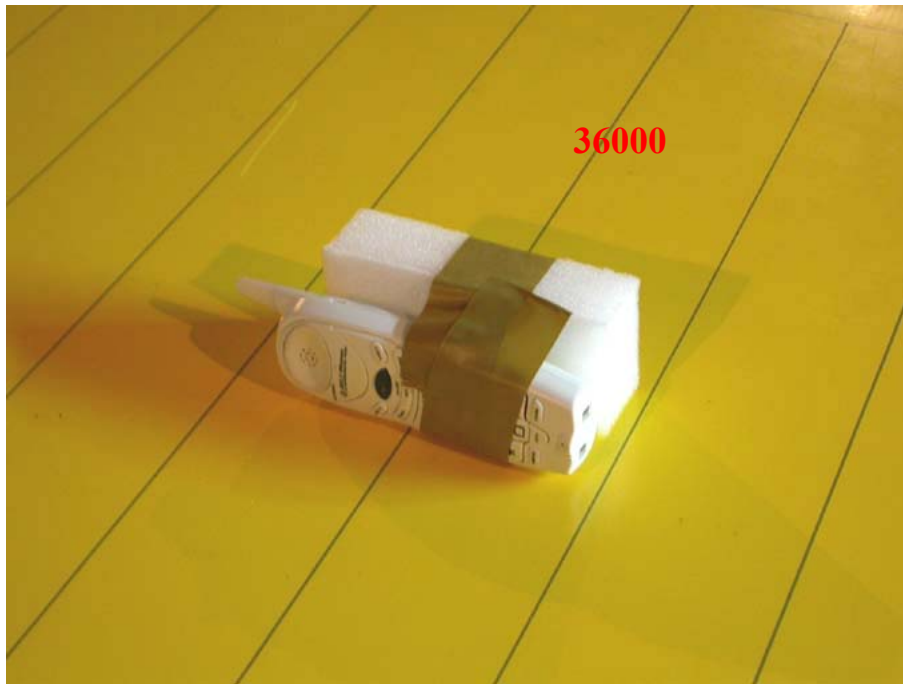
Photo 5: Radiated Emission Test Set-up photo (Handset)
