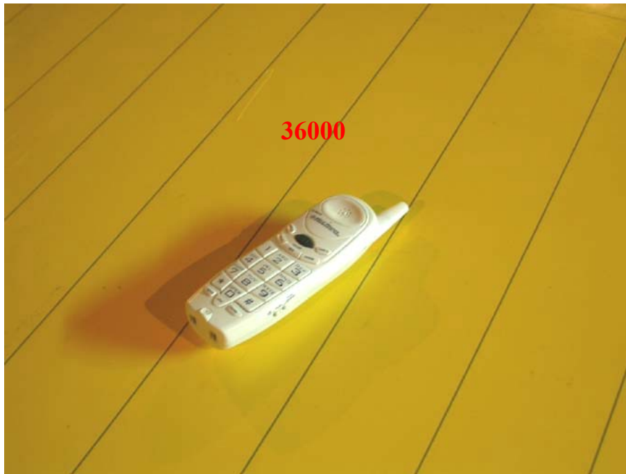
Photo 3: Radiated Emission Test Set-up photo (Handset)
