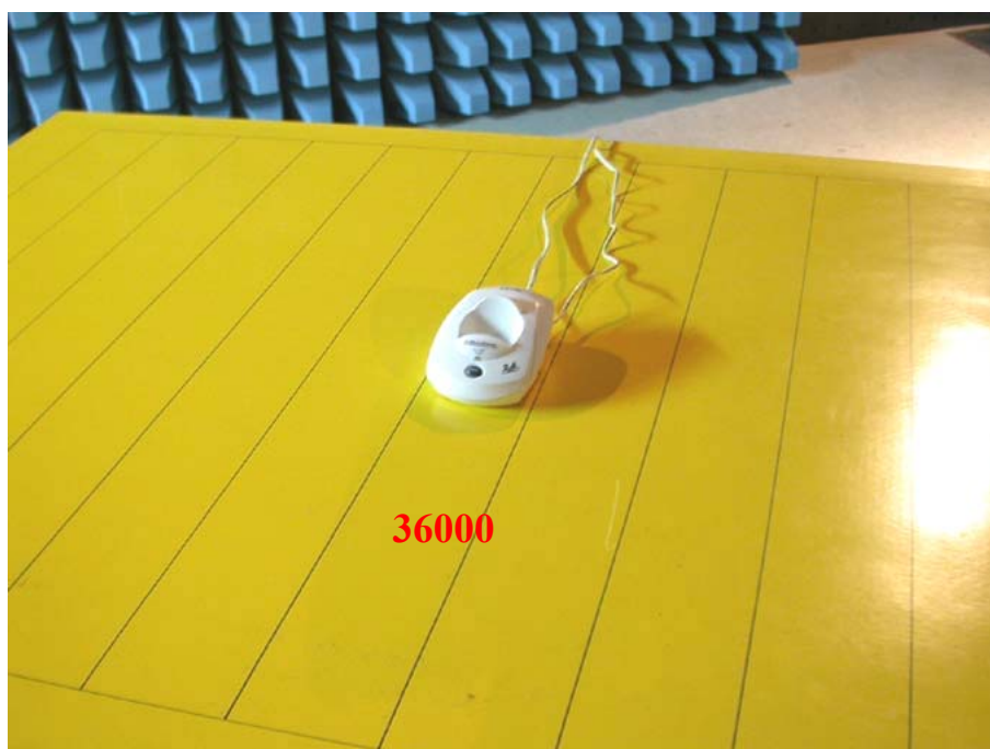
Photo 1: Radiated Emission Test Set-up photo (Base)
