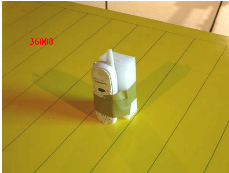
Photo 4: Radiated Emission Test Set-up photo (Handset)
