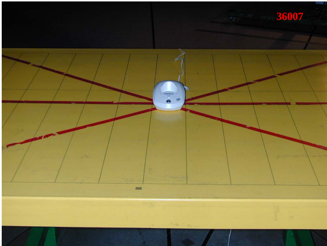
Photo 1: Radiated Emission Test Set-up photo (Base)
