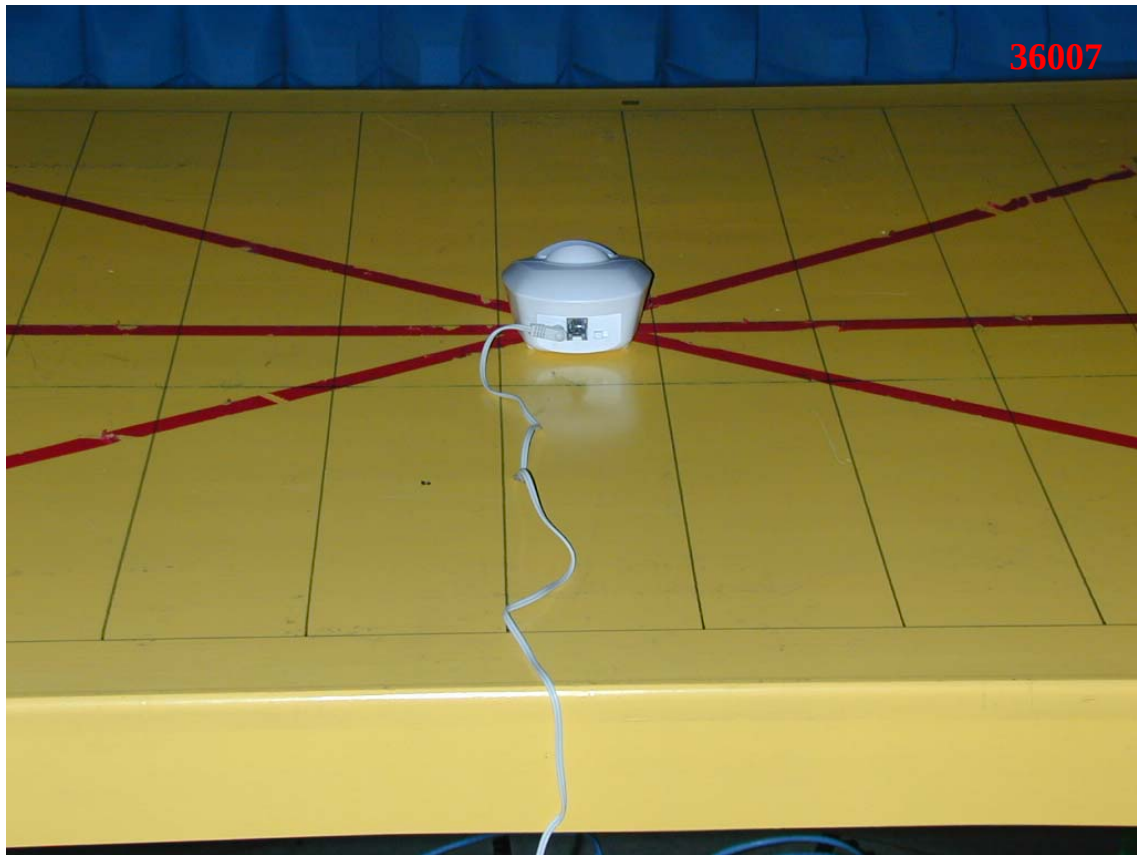
Photo 2: Radiated Emission Test Set-up photo (Base)
