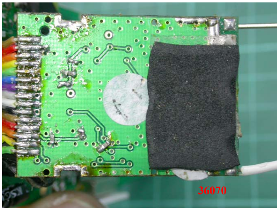
Photo 23: Internal photo of EUT (Handset)
