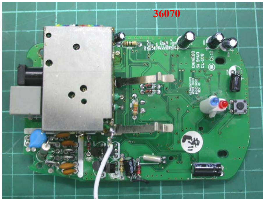
Photo 3: Internal photo of EUT (Base)
