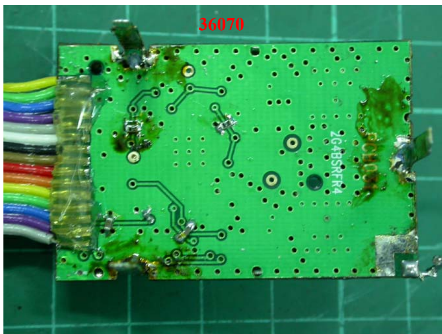
Photo 8: Internal photo of EUT (Base)
