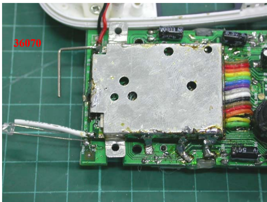
Photo 18: Internal photo of EUT (Handset)
