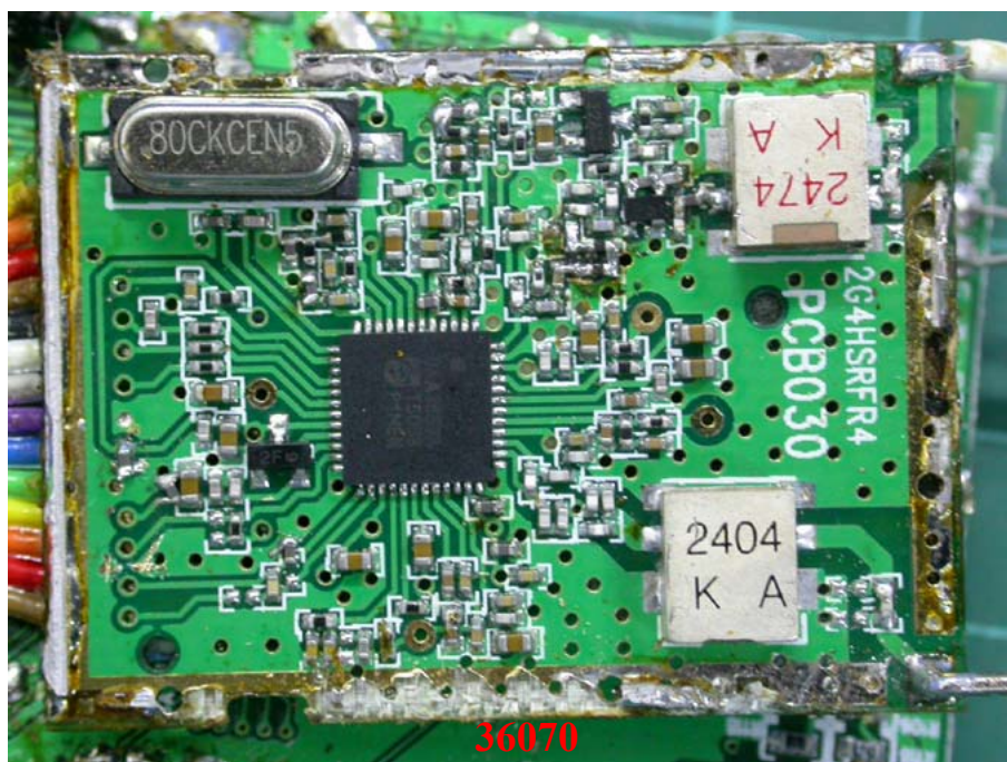
Photo 22: Internal photo of EUT (Handset)
