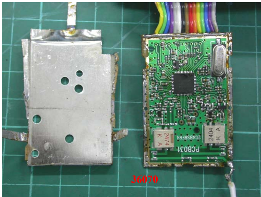
Photo 9: Internal photo of EUT (Base)
