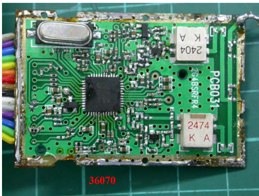
Photo 10: Internal photo of EUT (Base)
