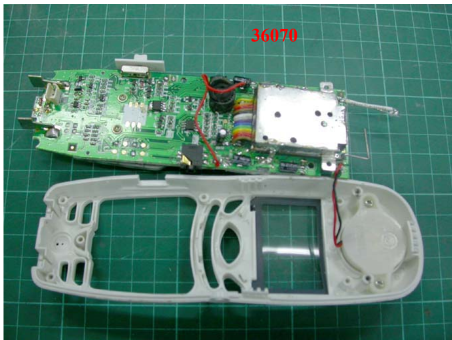
Photo 15: Internal photo of EUT (Handset)
