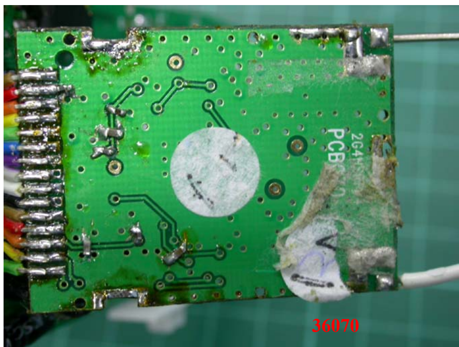
Photo 24: Internal photo of EUT (Handset)
