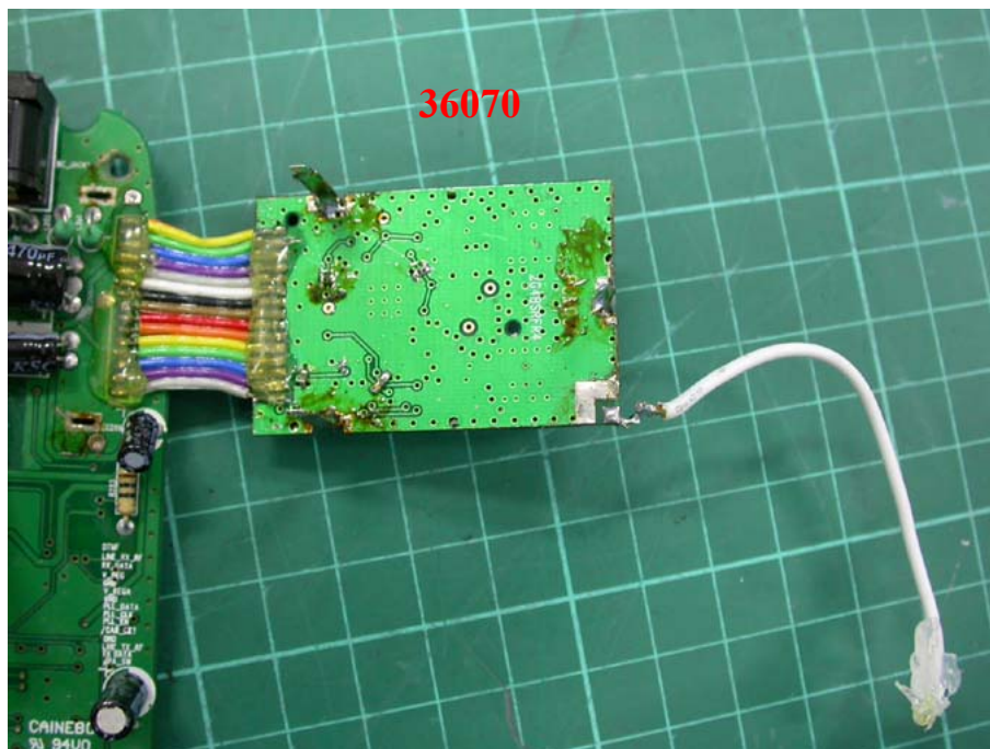
Photo 7: Internal photo of EUT (Base)
