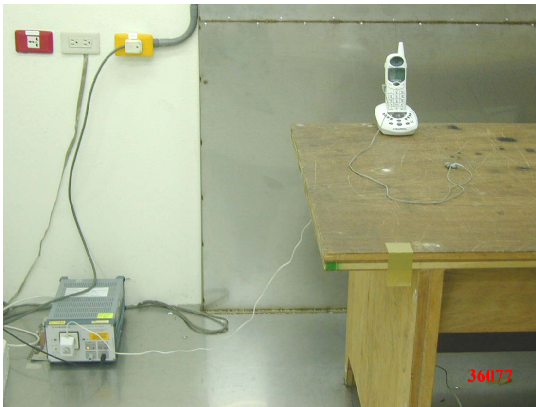
Photo 1: Conducted Emission Test Set-up photo (Handset with Base)
