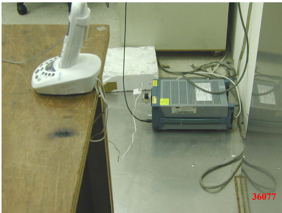
Photo 2: Conducted Emission Test Set-up photo (Handset with Base)
