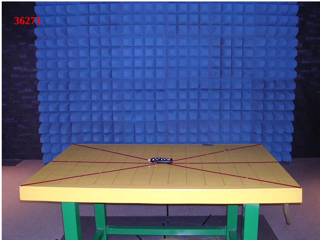
Photo 4: Radiated Emission Test Set-up photo (Handset)
