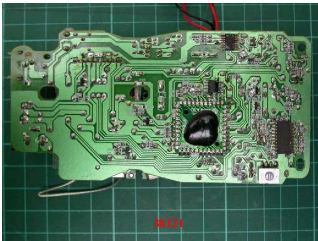
Photo 26: Internal photo of Series model (Base)
