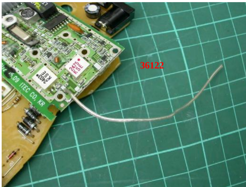
Photo 14: Internal photo of EUT (Base)
