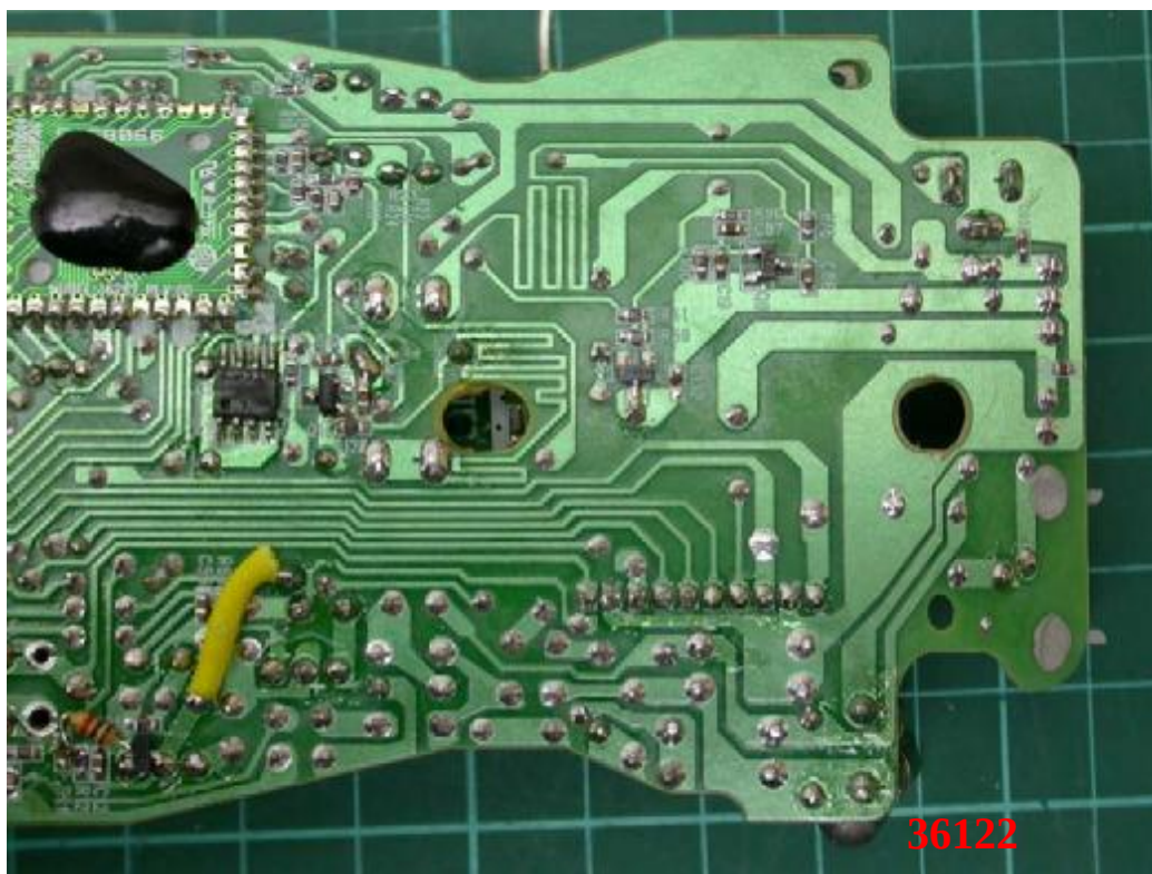
Photo 13: Internal photo of EUT (Base)
