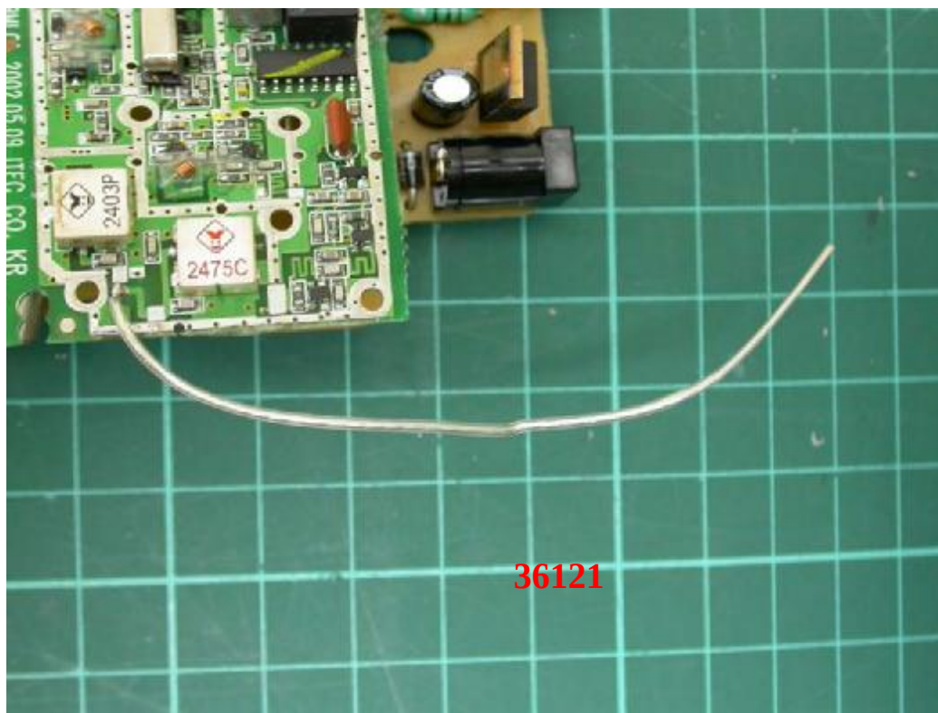
Photo 33: Internal photo of Series model (Base)
