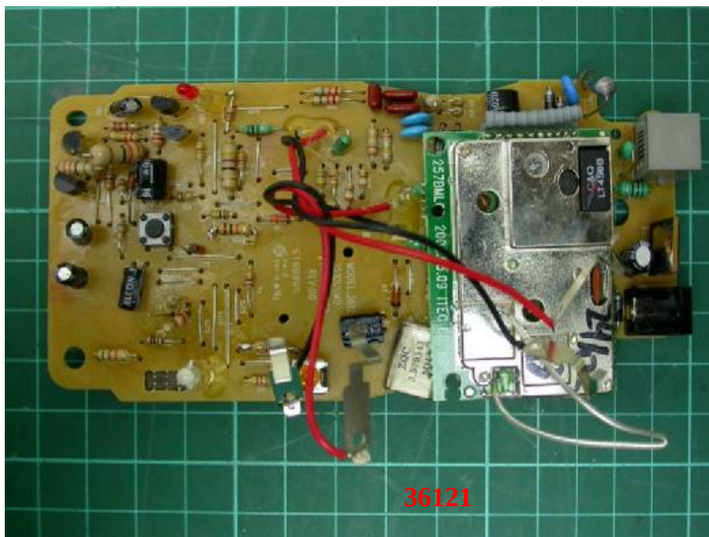
Photo 22: Internal photo of Series model (Base)
