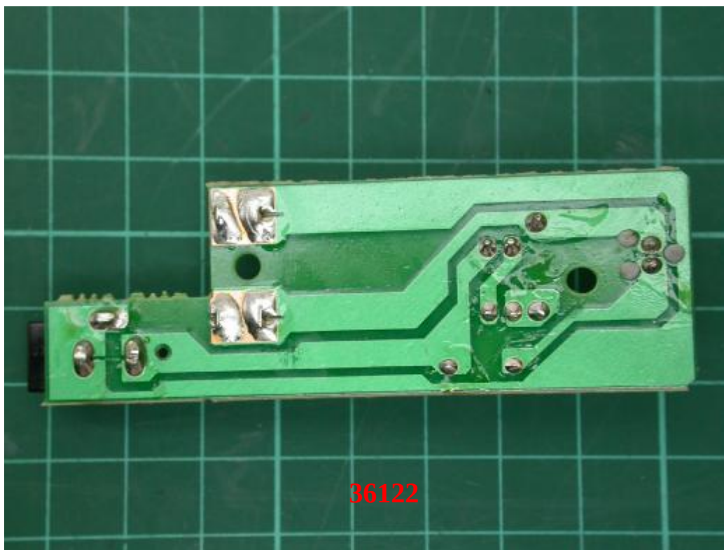
Photo 18: Internal photo of EUT (Base)
