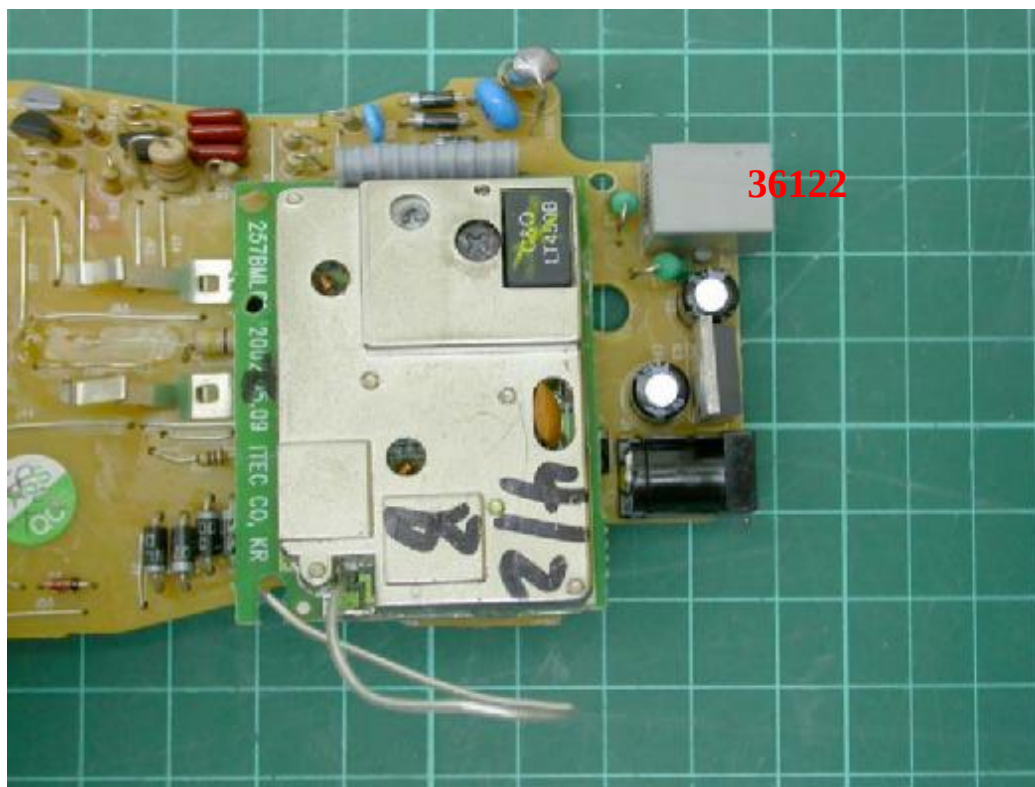
Photo 5: Internal photo of EUT (Base)
