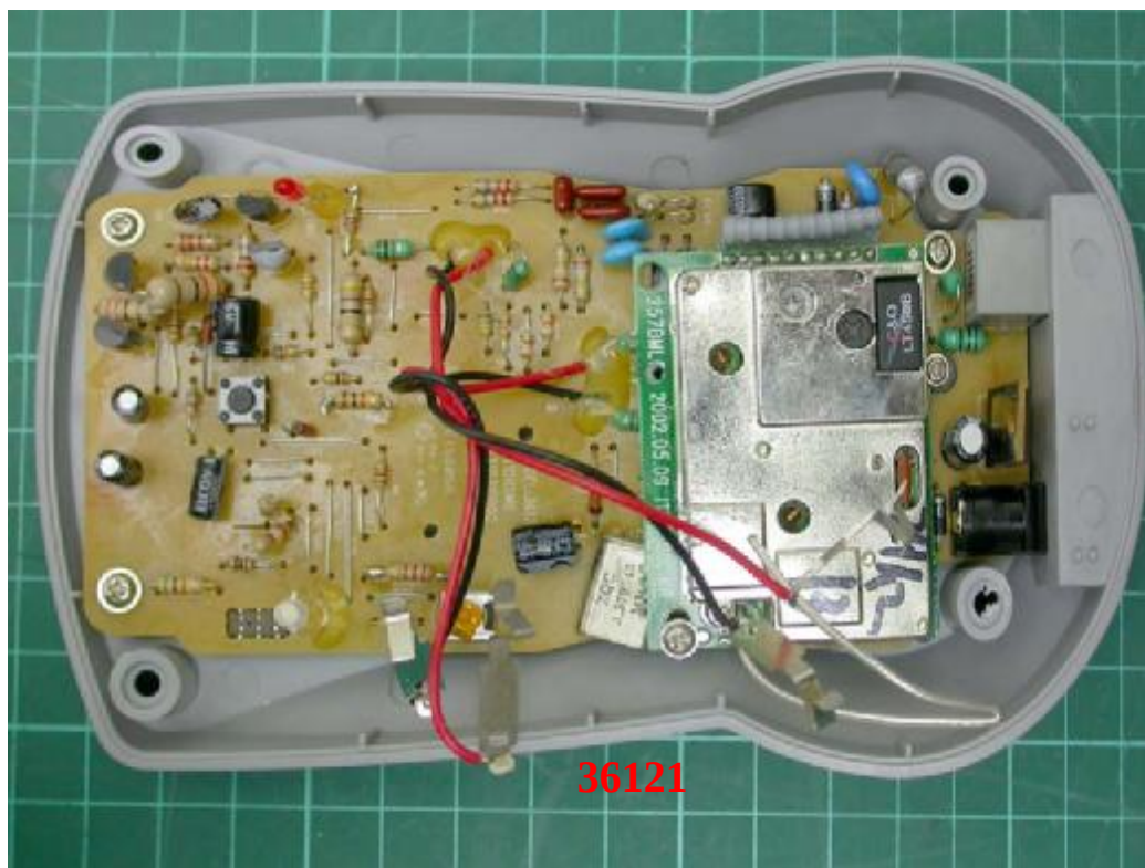
Photo 21: Internal photo of Series model (Base)
