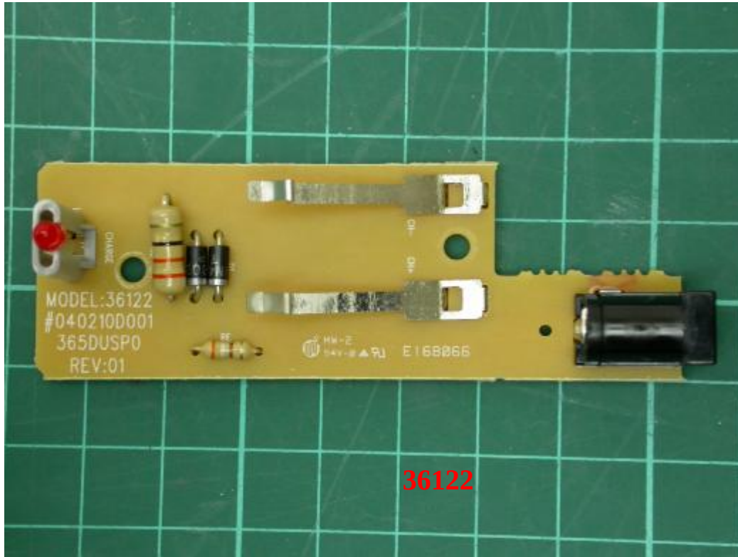
Photo 17: Internal photo of EUT (Base)
