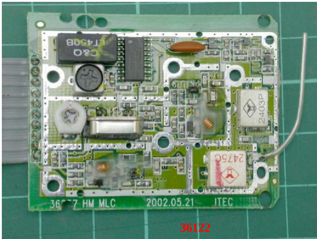
Photo 13: Internal photo of EUT (Handset)
