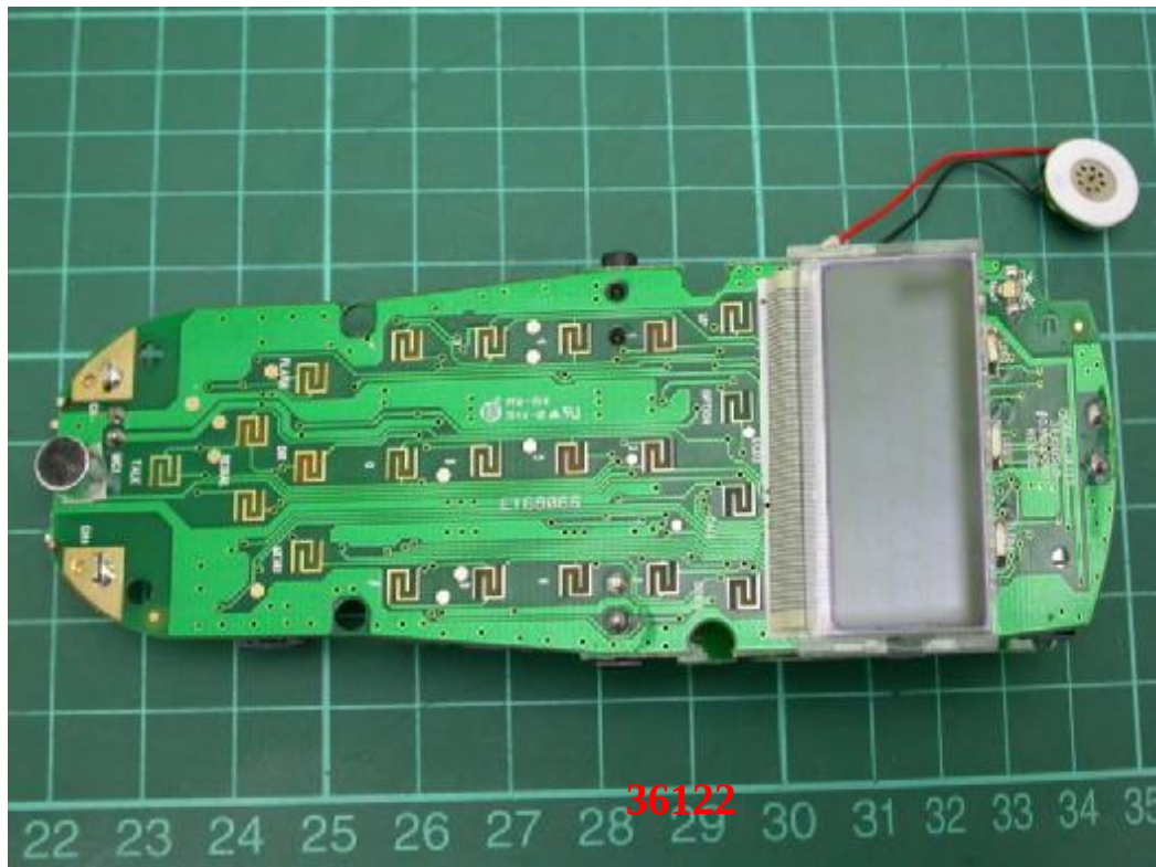
Photo 8: Internal photo of EUT (Handset)
