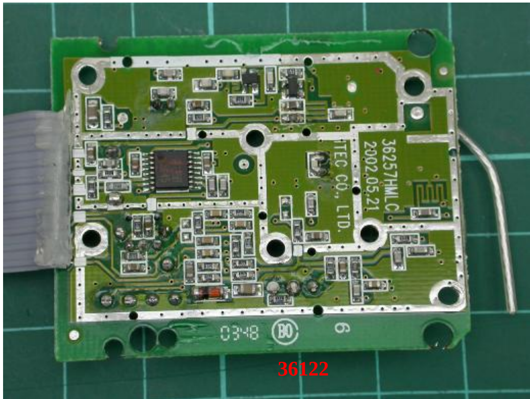
Photo 14: Internal photo of EUT (Handset)
