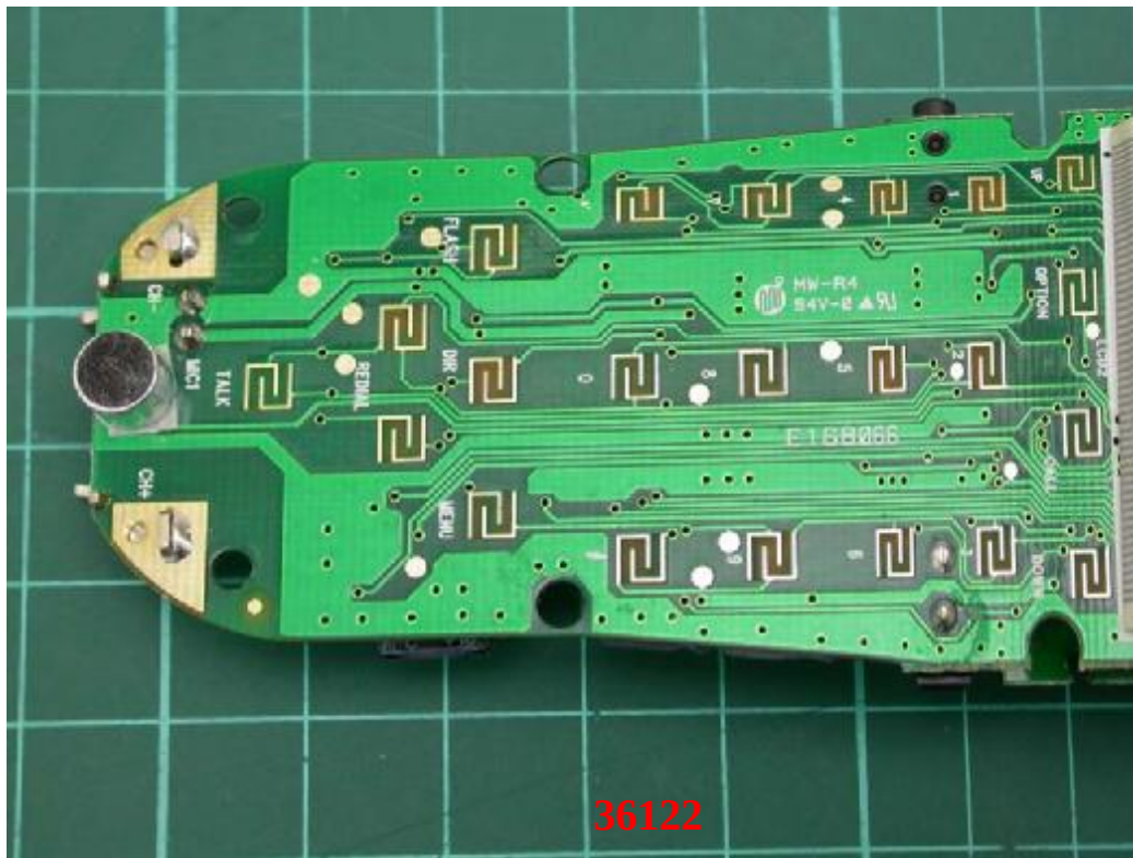
Photo 10: Internal photo of EUT (Handset)
