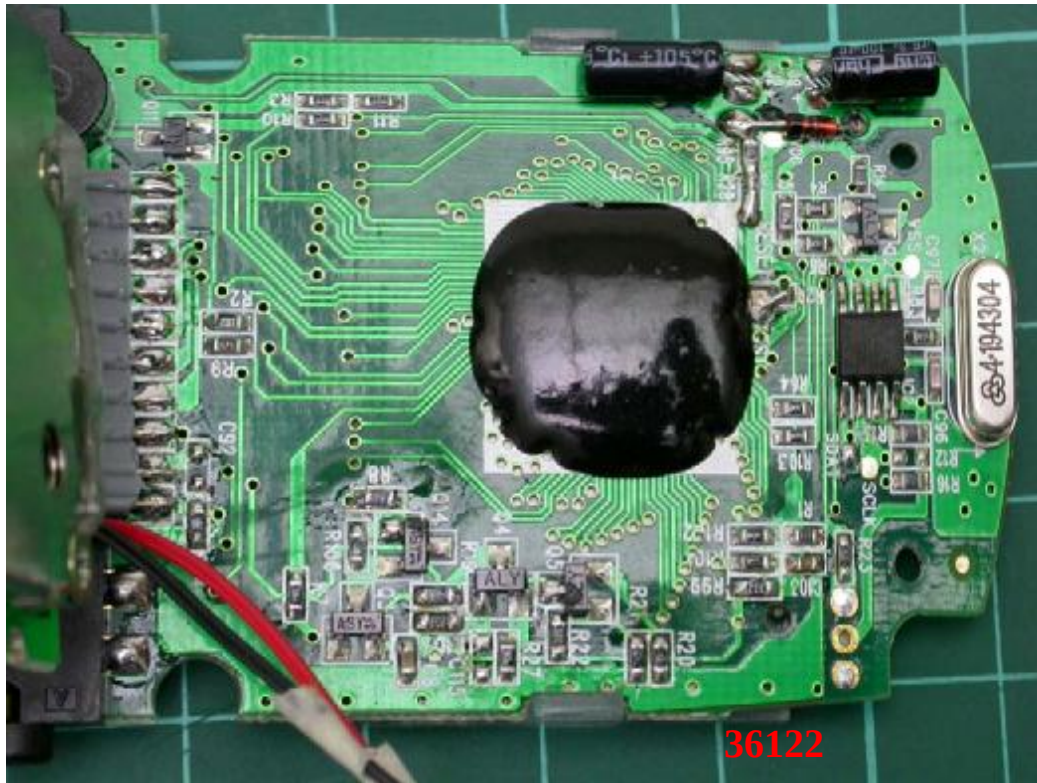
Photo 7: Internal photo of EUT (Handset)
