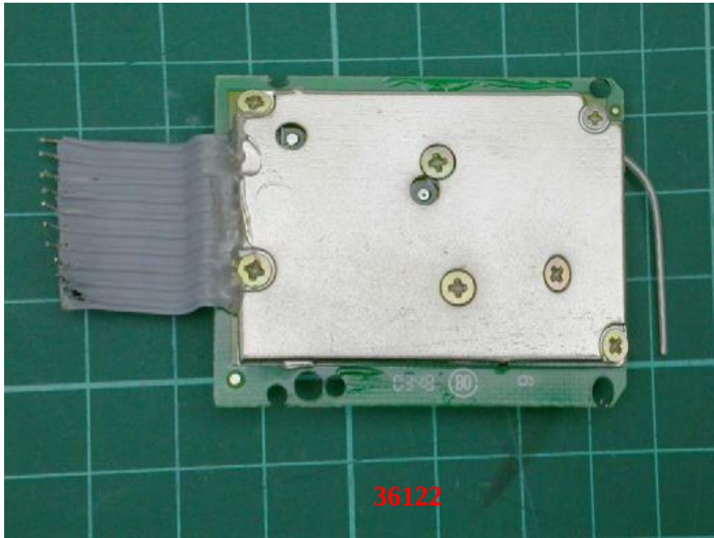
Photo 12: Internal photo of EUT (Handset)
