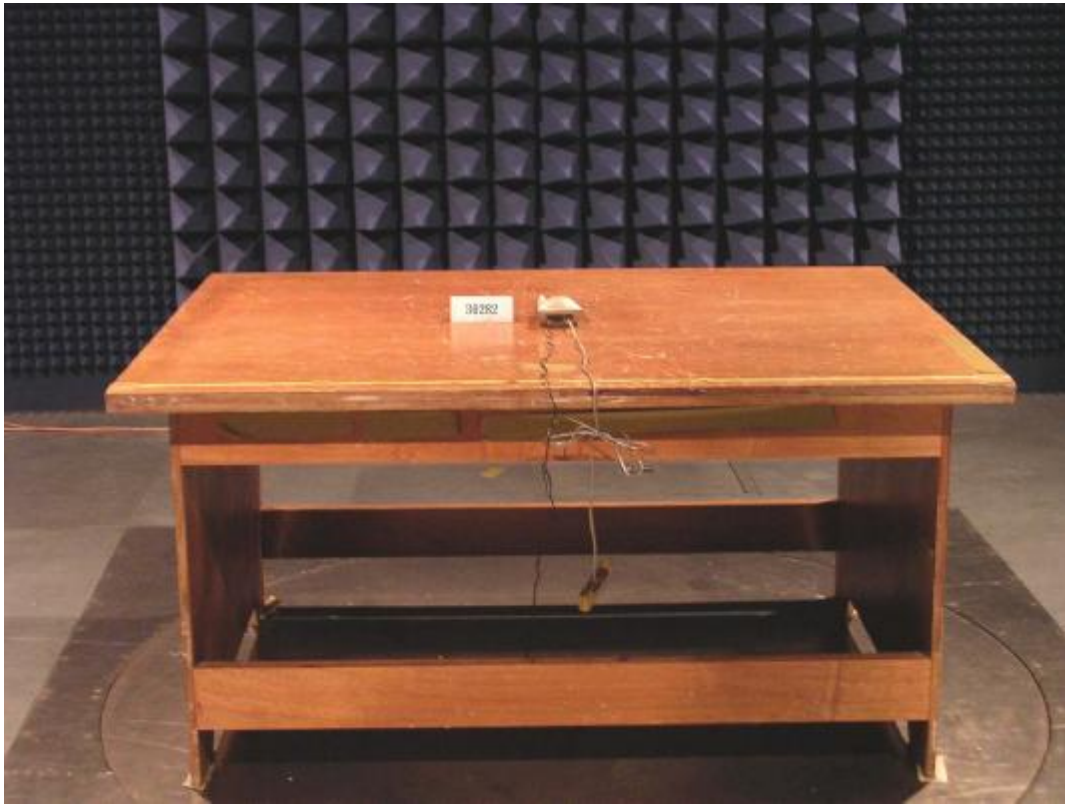
Photo 2: Radiated Emission Test Set-up (Base Unit)
