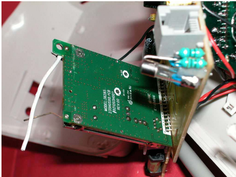
Base Oscillator PCB solder side (view 1)
