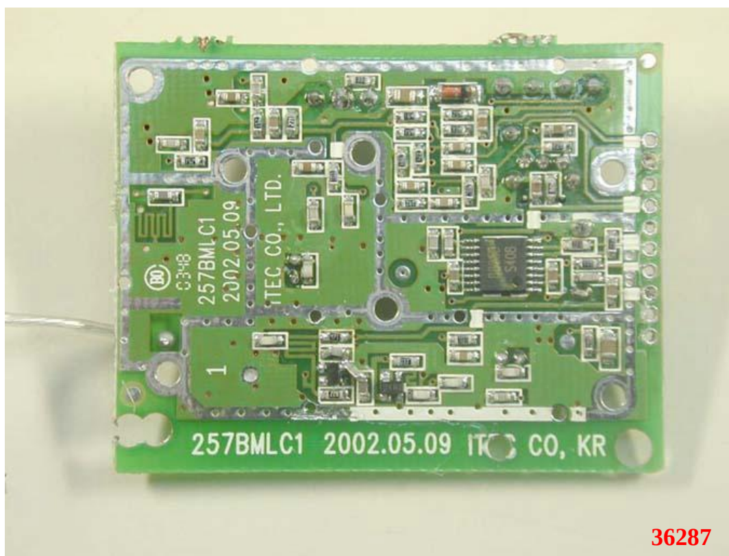
Photo 8: Internal photo of EUT (Base)
