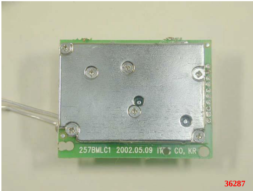
Photo 7: Internal photo of EUT (Base)
