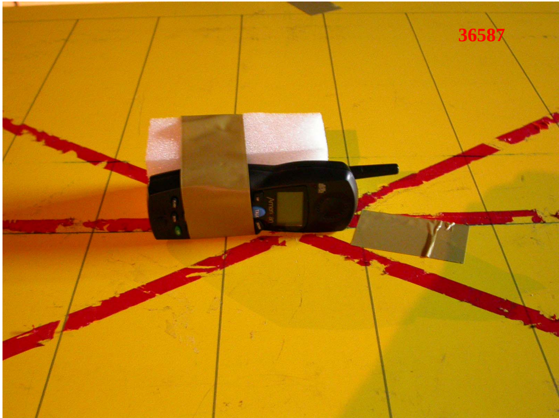
Photo 5: Radiated Emission Test Set-up photo
