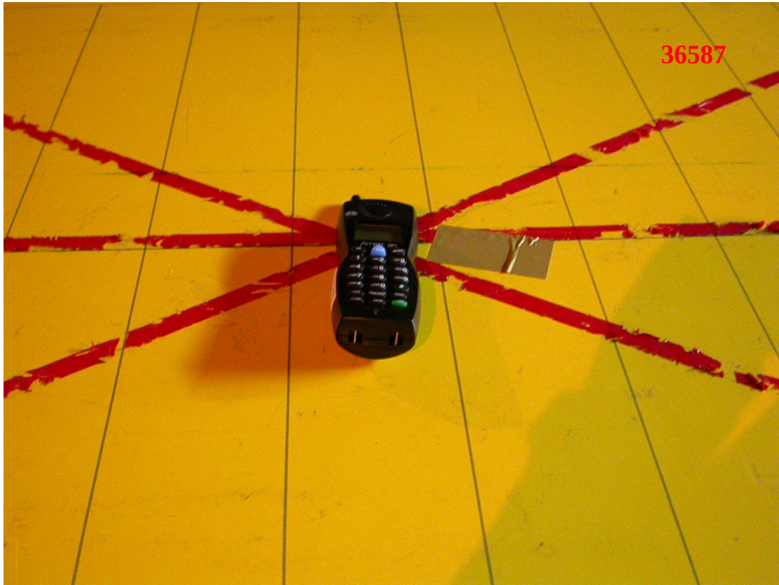
Photo 3: Radiated Emission Test Set-up photo
