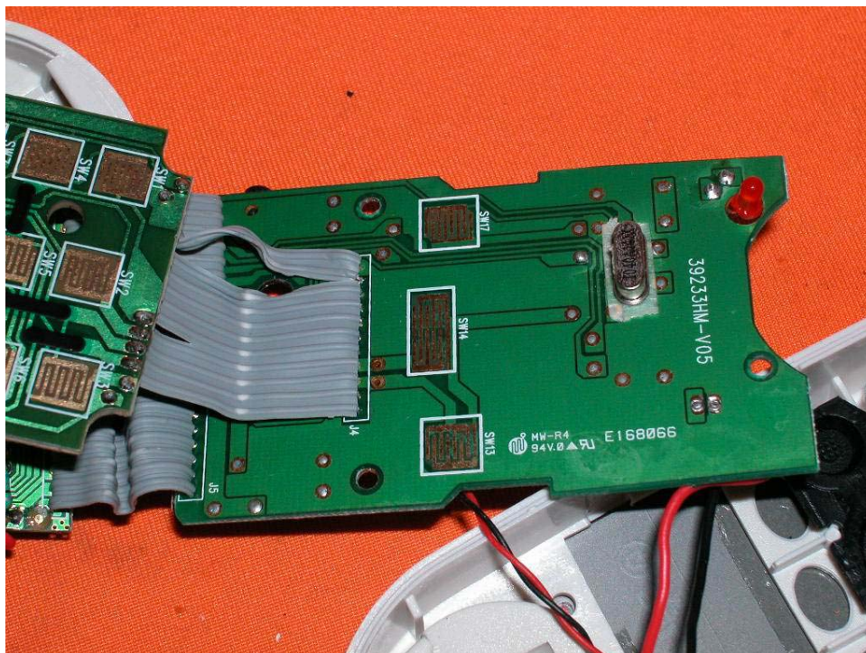
Handset Main PCB keypad side (View 1)
