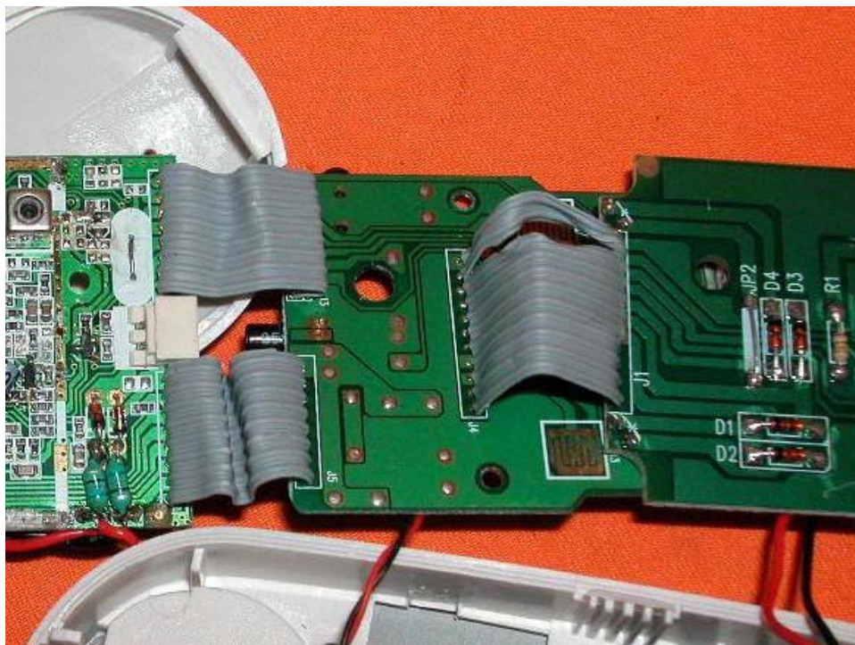
Handset Main PCB keypad side (View 2)
