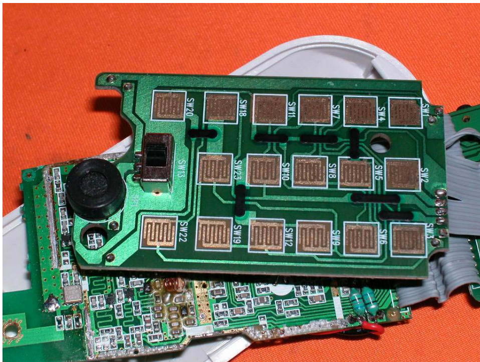
Handset Main PCB keypad side (View 3)
