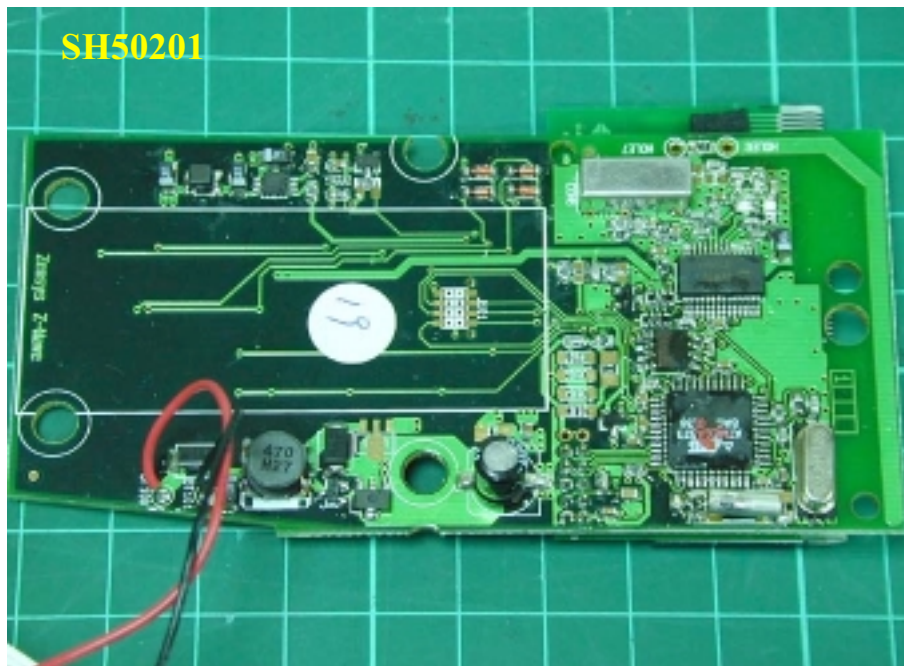
Photo 2: Inner view
