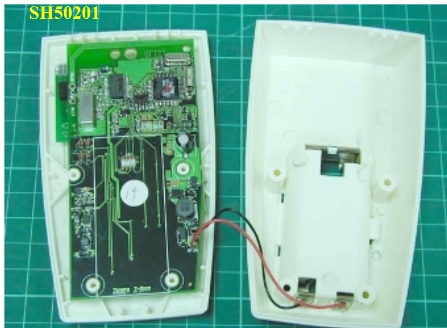
Photo 1: Inner view
