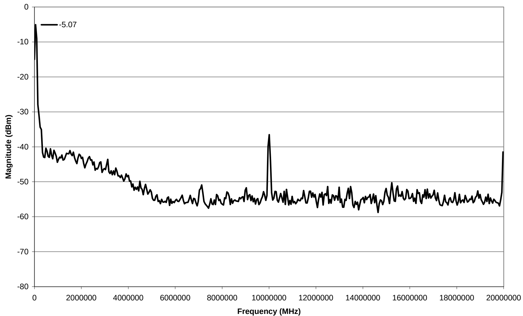
SAM016 Receiver Baseband Signal FFT (-60 dBm Input, 2X Info BW)
