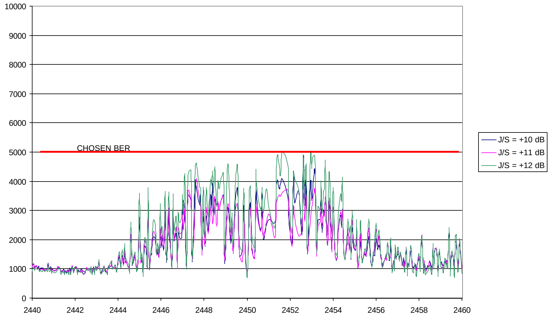
SAM019 Receiver BER - Errors per 100,000 bits (Combined DSSS Input & Jammer Input) 15.3% of Jammer frequencies discarded
