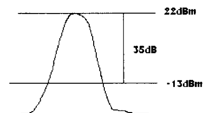
Figure 9.1. Drawing of the limit line calculated from the maximum signal power of the EUT.
