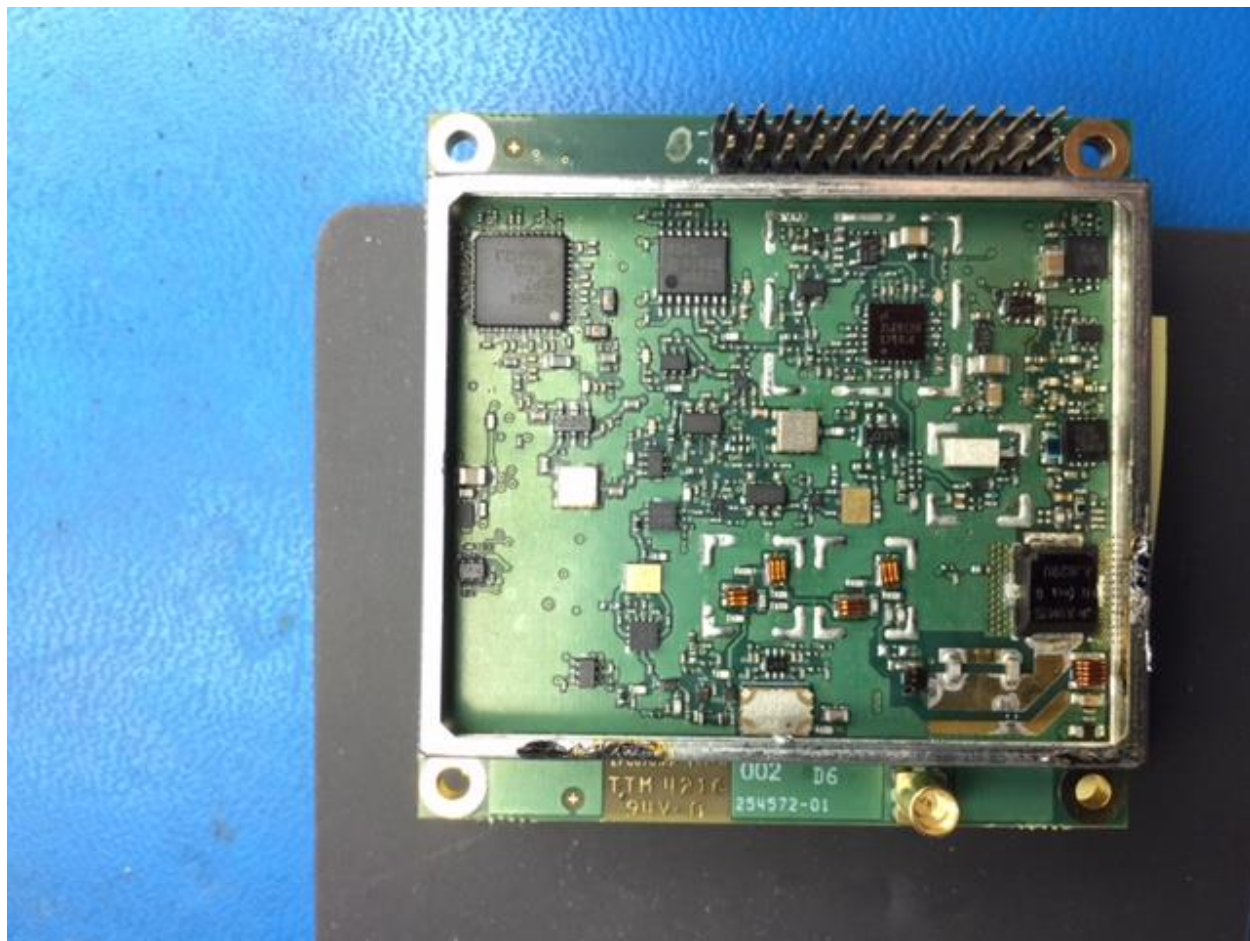
PHOTO: TOP SIDE XETA7-M2 WITHOUT SHIELD
