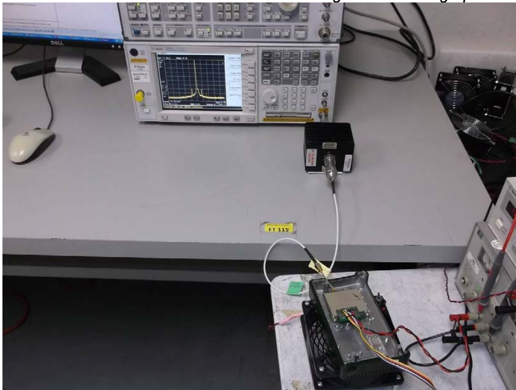
RF Conducted Measurements Test Configuration Photographs
