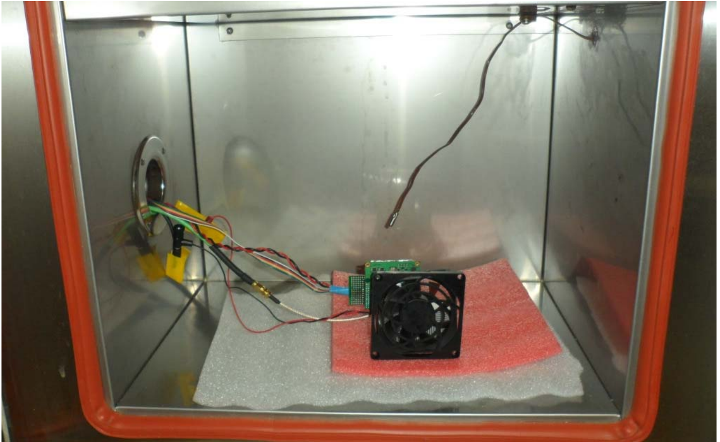
Figure E21.5 – Setup Photo – Frequency Stability Measurements
