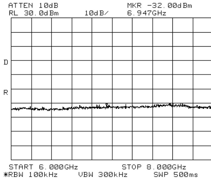
Spurious BPSK 6GHz – 8GHz, high
