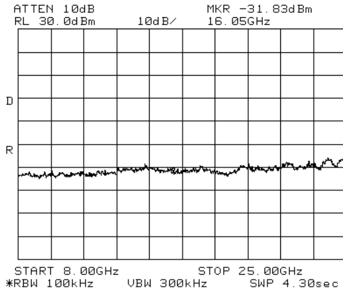
Spurious 32QAM 8GHz – 25GHz, low
