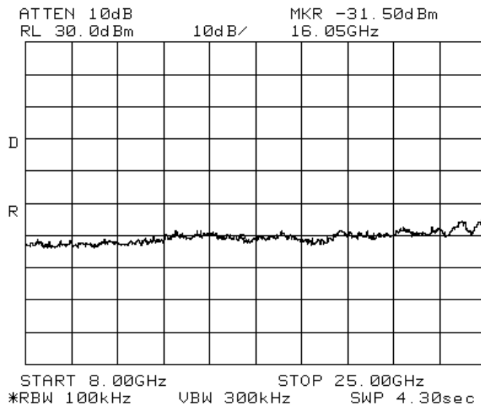
Spurious QPSK 8GHz – 25GHz, high
