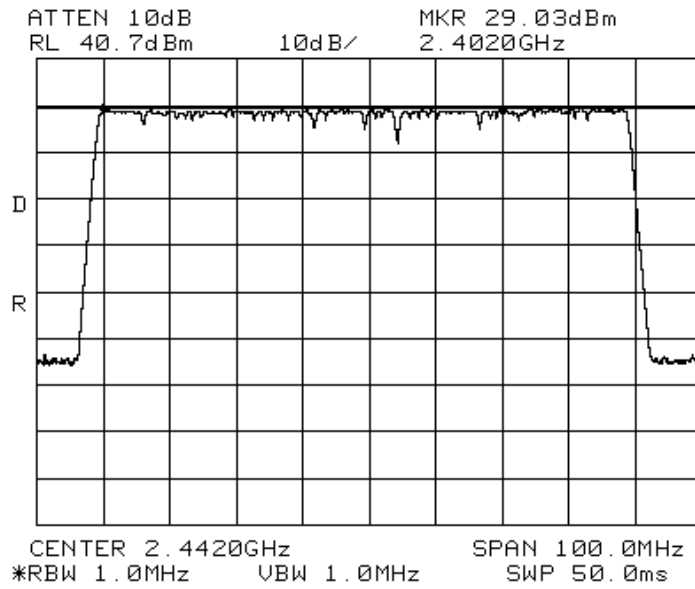
RF Power Output 57 kbps Low 2401.74 MHz
