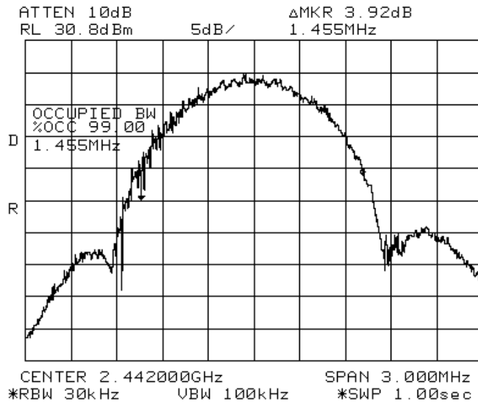
8PSK mid 99% OBW
