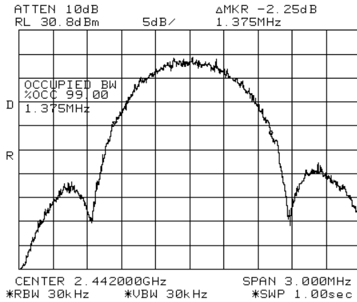
QPSK mid 99% OBW
