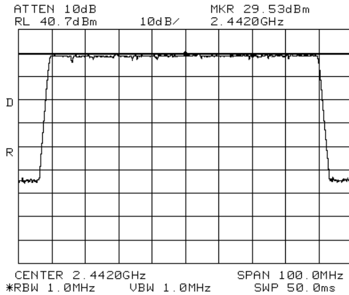
RF Power Output 57 kbps mid 2442 MHz
