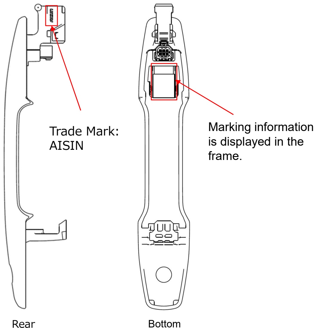
Figure 12 Marking layout
