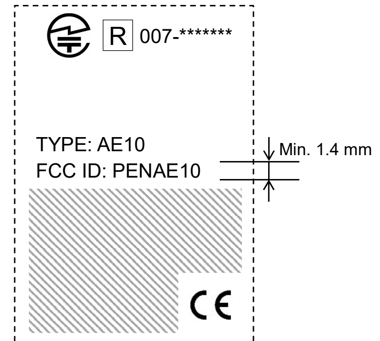
Figure 13 Marking information
