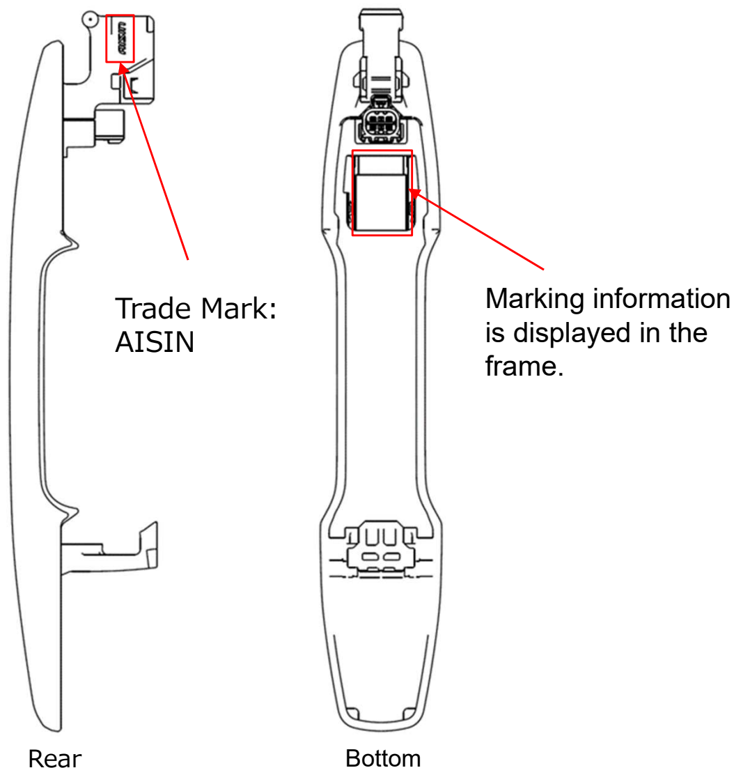
Figure 12 Marking layout
