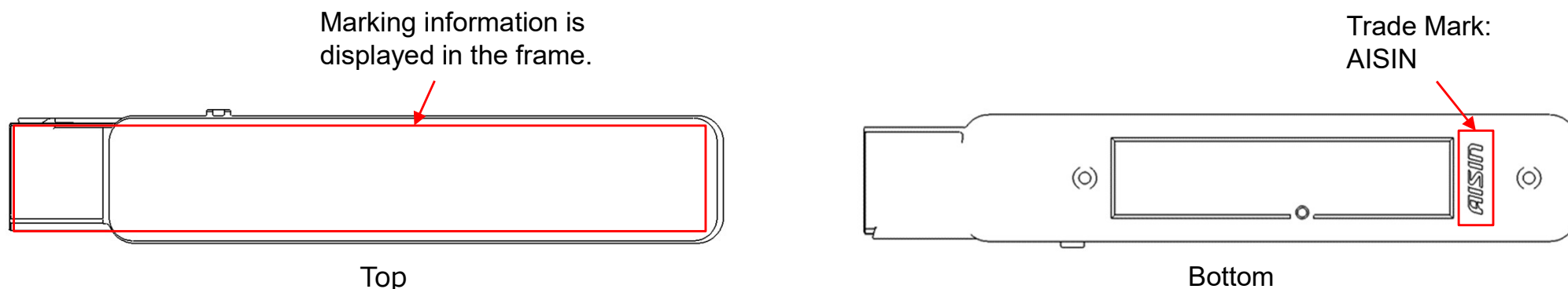
Figure 10 Marking layout
