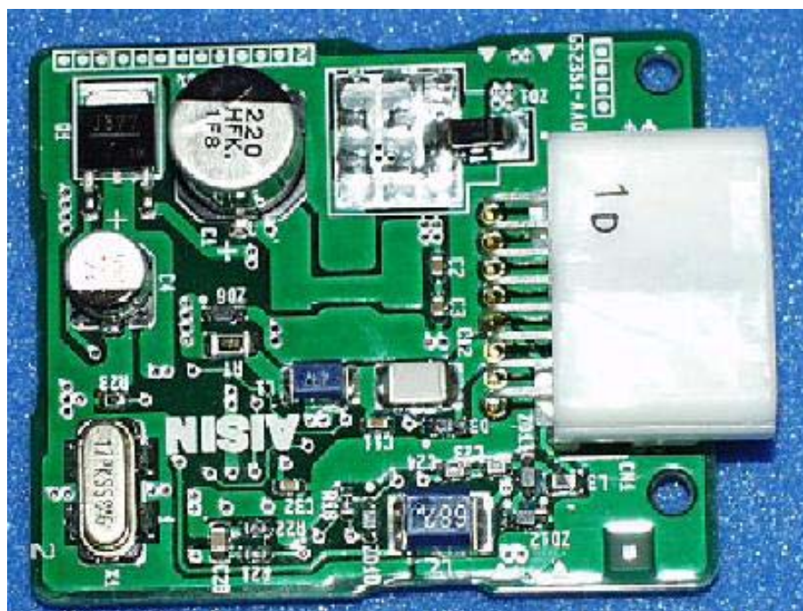
Oscillator Circuit Board (front)
