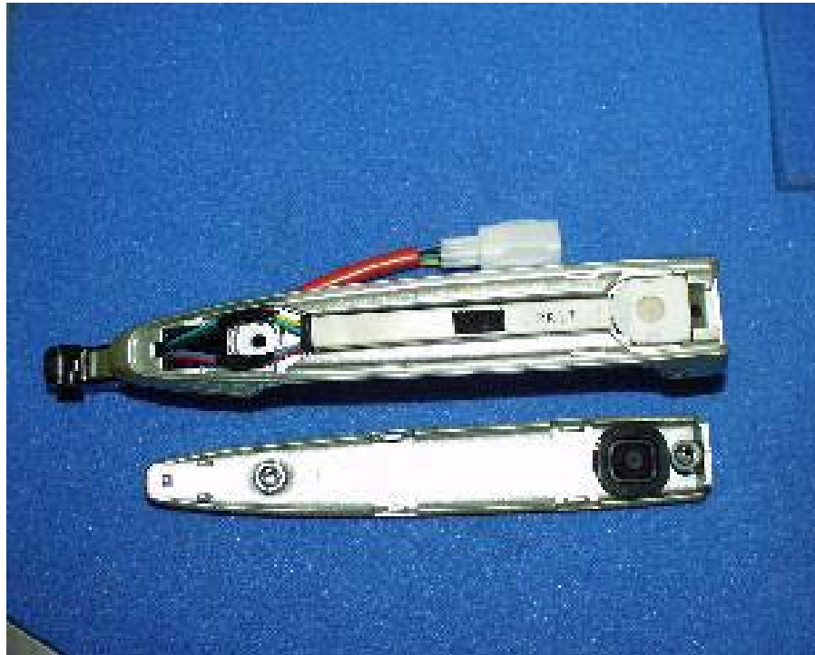
Internal View of Door Antenna (Large)
