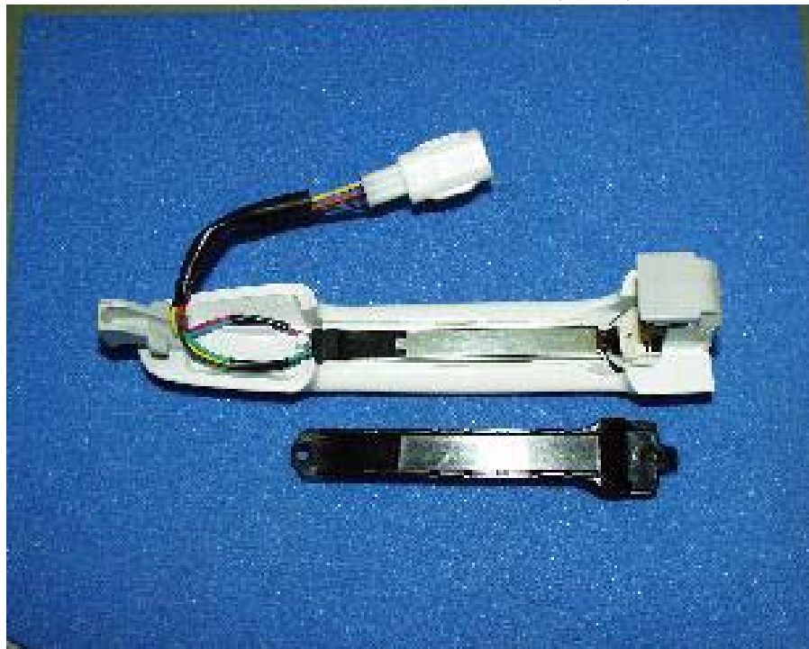
Internal View of Door Antenna (Small)
