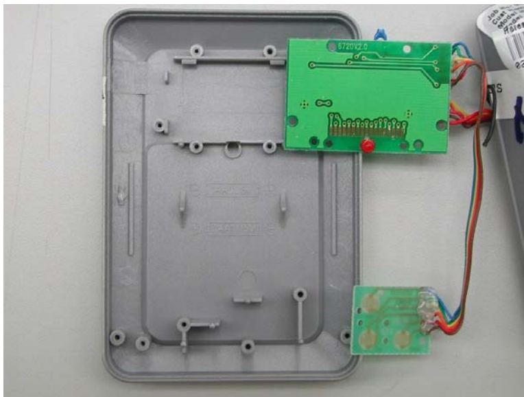
Internal Photo – 4
