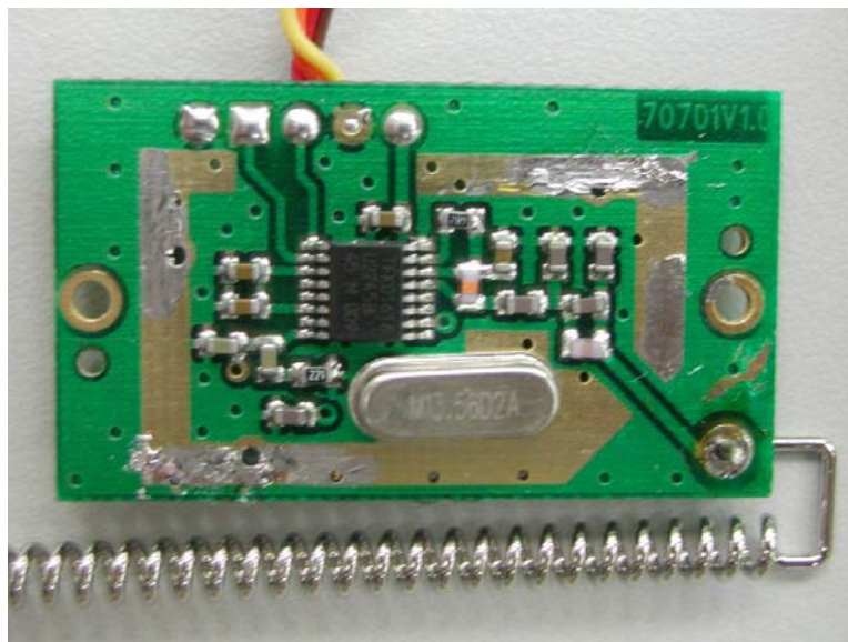
Internal Photo – 6
