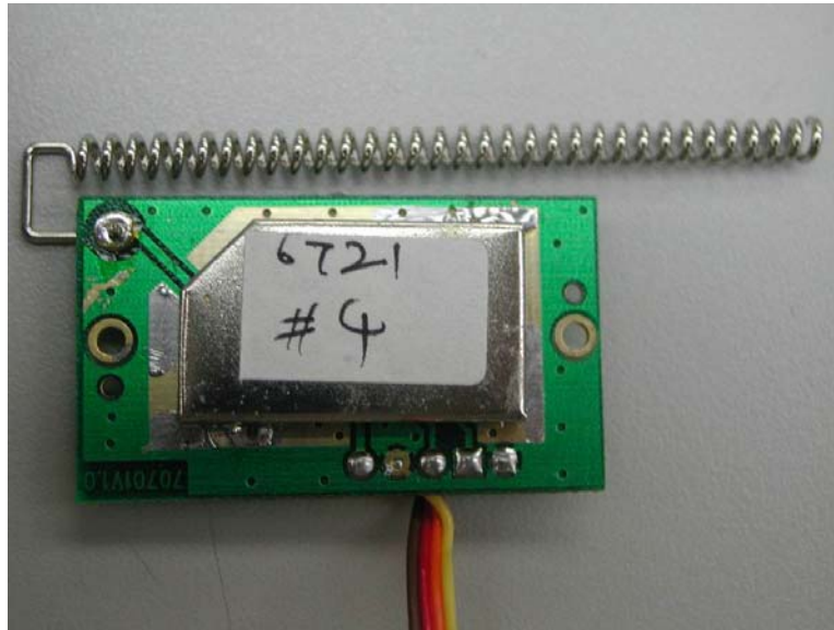
Internal Photo – 6
