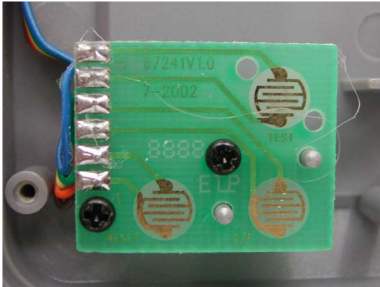
Internal Photo – 3
