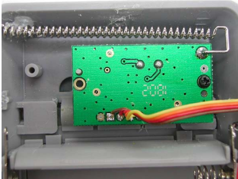
Internal Photo – 7
