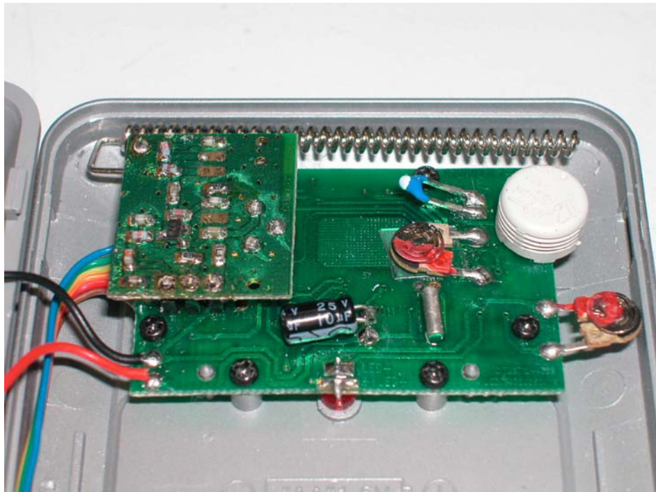
Internal Photo - 2
