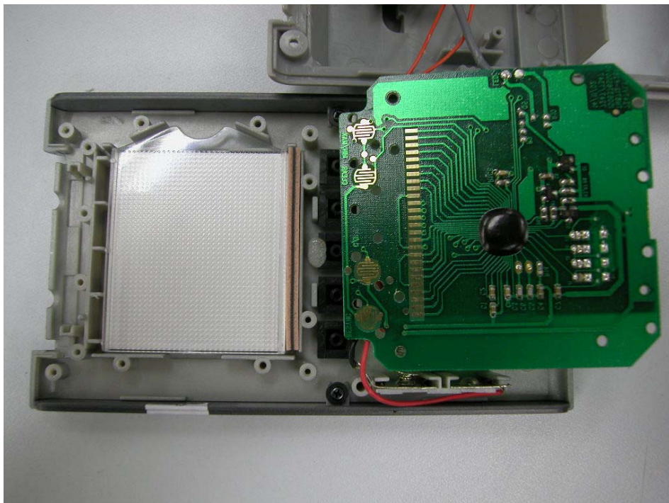
Internal Photo – 8 (model: 7249 without back light)
