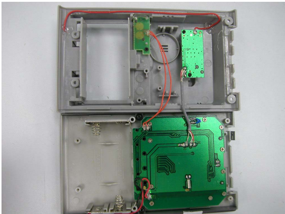
Internal Photo – 2 (model: 7249 without back light)
