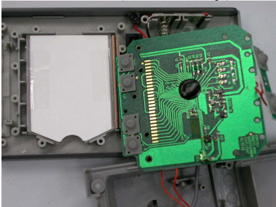
Internal Photo – 7 (model:7247 with back light)
