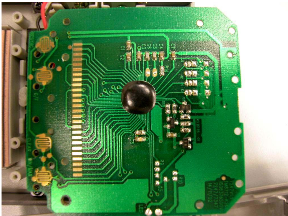
Internal Photo – 10 (model: 7249 without back light)
