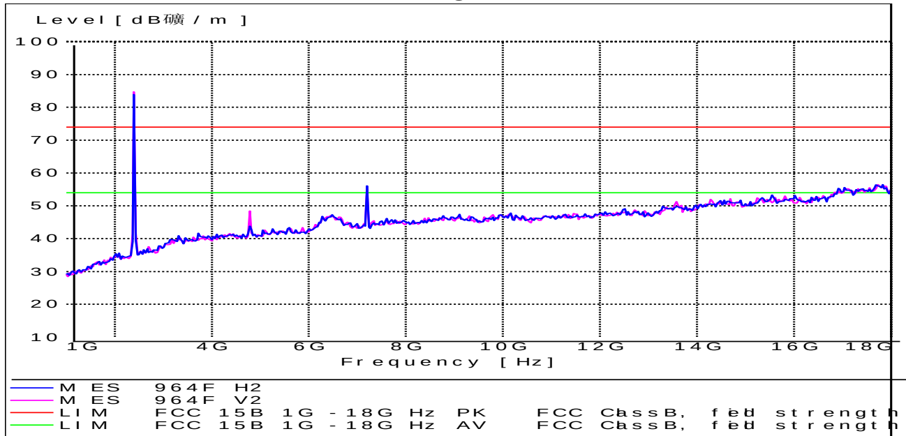
Channel 00 @ 2402 MHz
