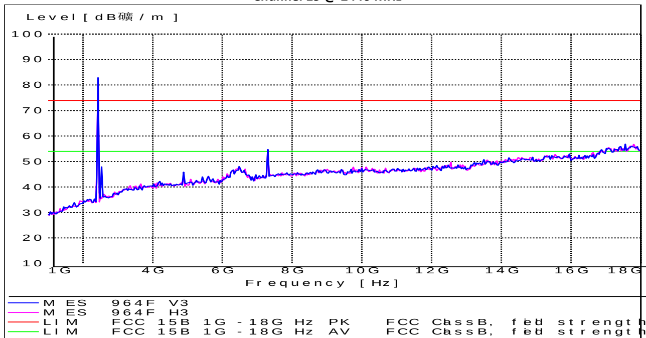
Channel 19 @ 2440 MHz
