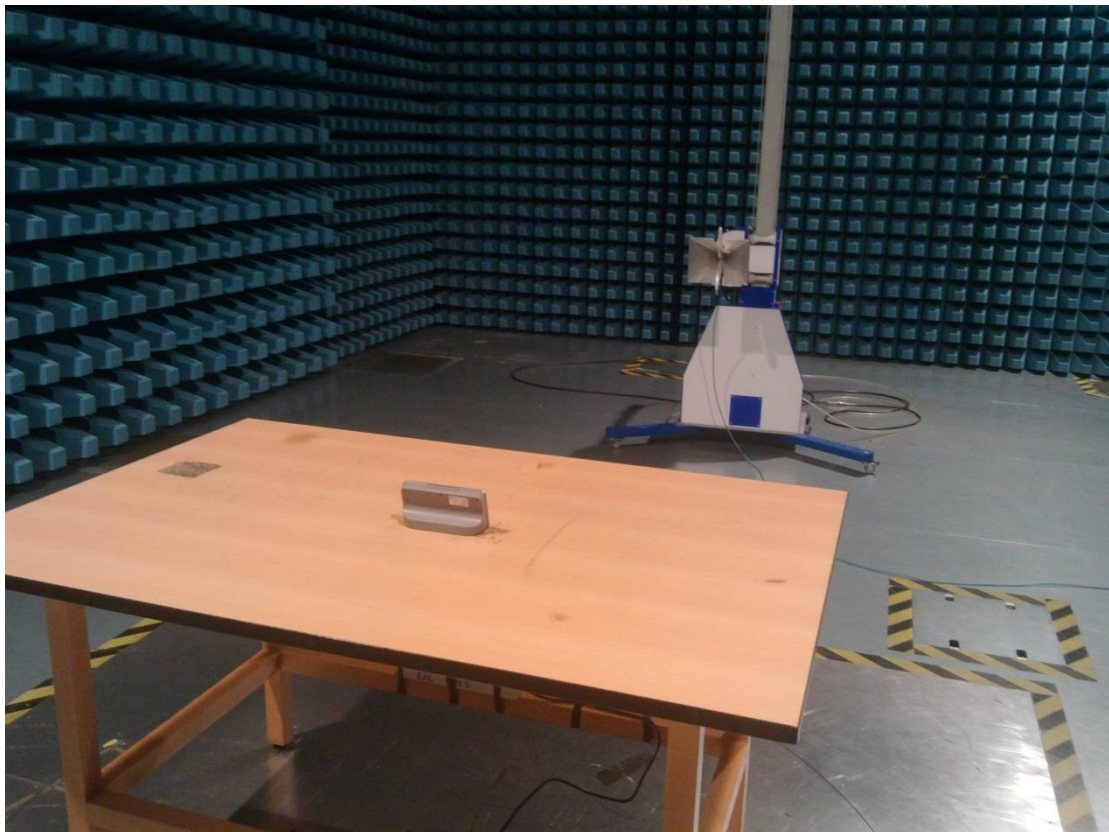
Above 1 GHz
