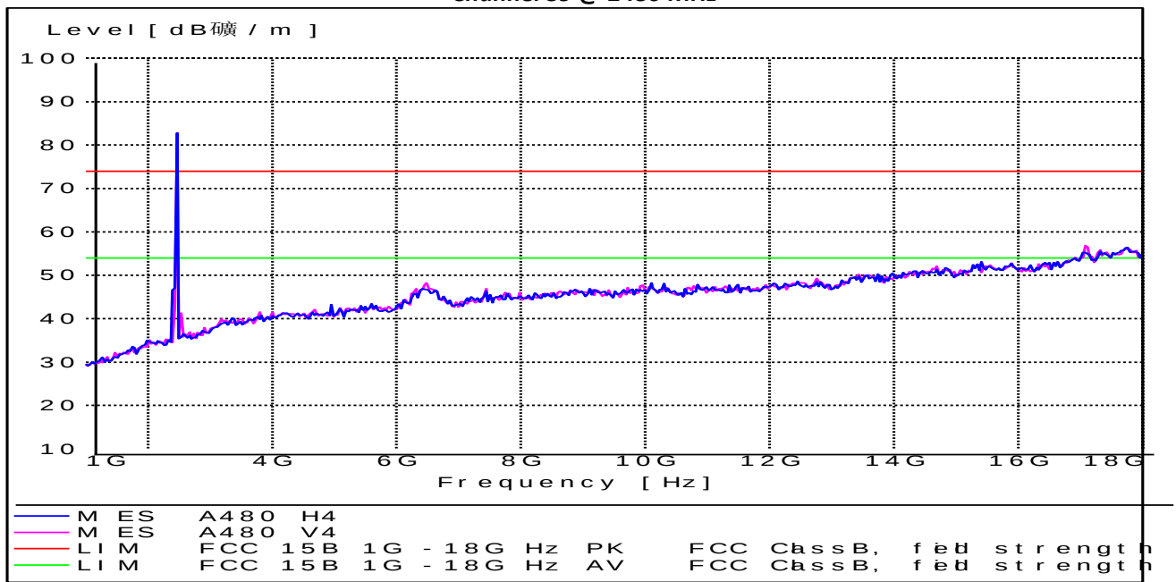
Channel 39 @ 2480 MHz
