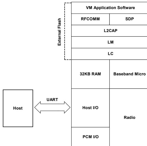
Figure 7.3: Virtual Machine
