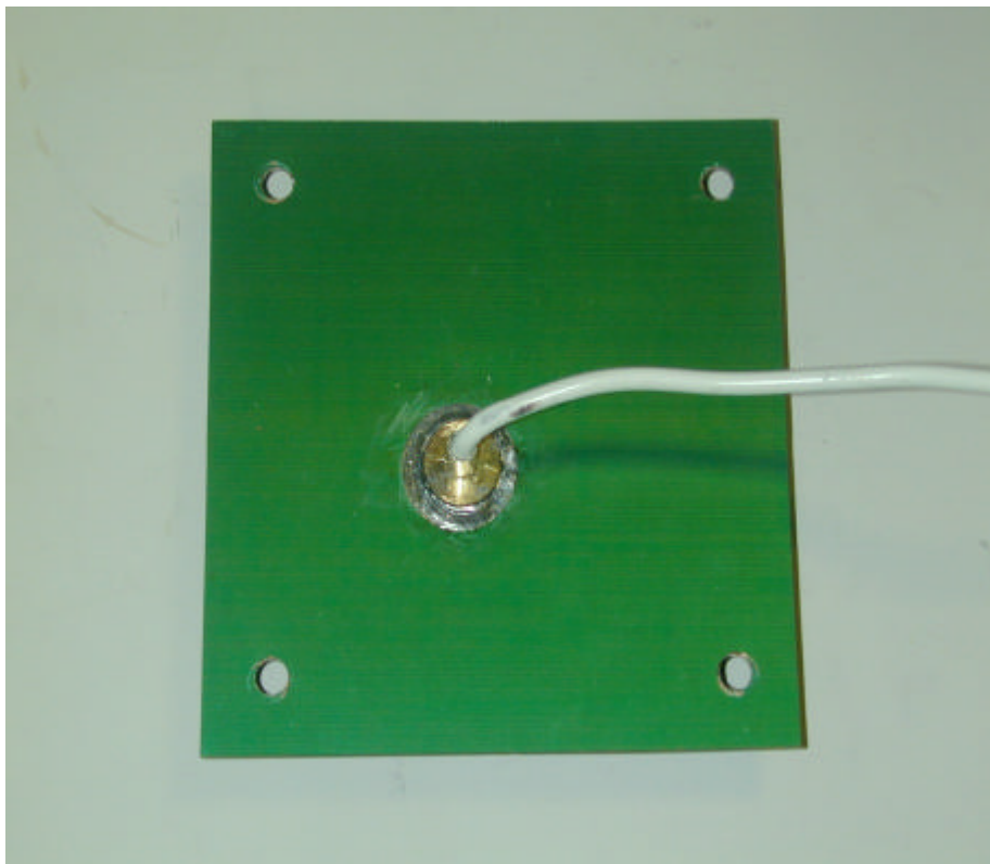
Internal View of 3000AS External Antenna, Bottom View of PCB.
