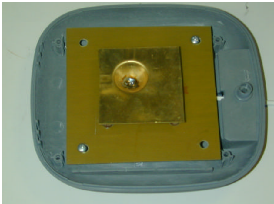
Internal View of 3000AS External Antenna, Top View of PCB.
