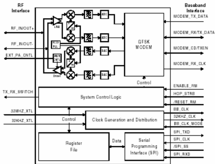
Figure 1: SW1502 IC Block Diagram
