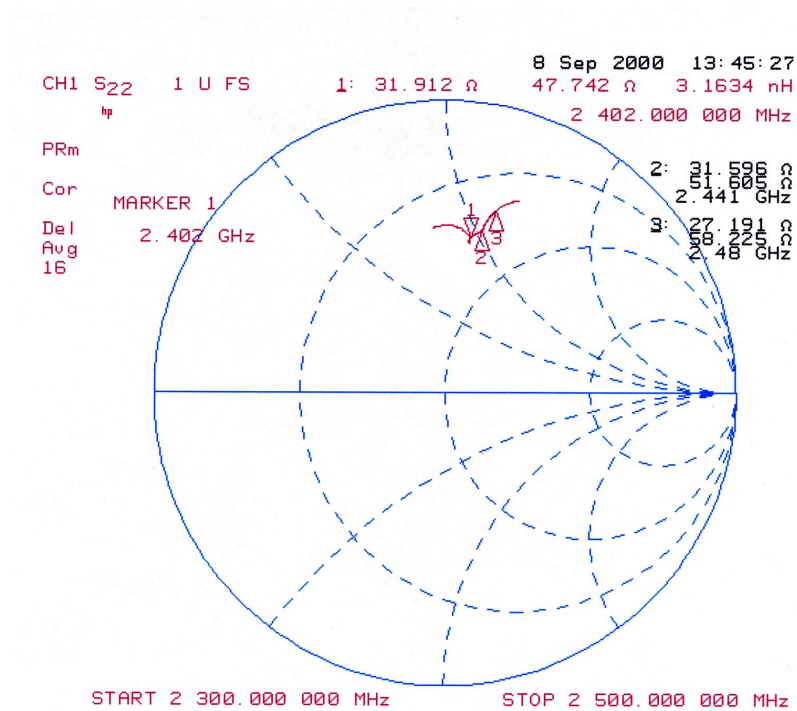
Figure 9: S22 Measurement from Pin 4
