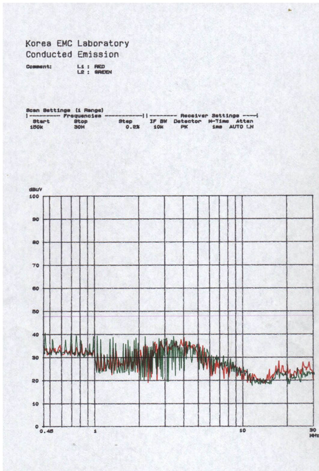
Red : HOT LINE, Green : Neutral LINE LINE EMISSION GRAPH
