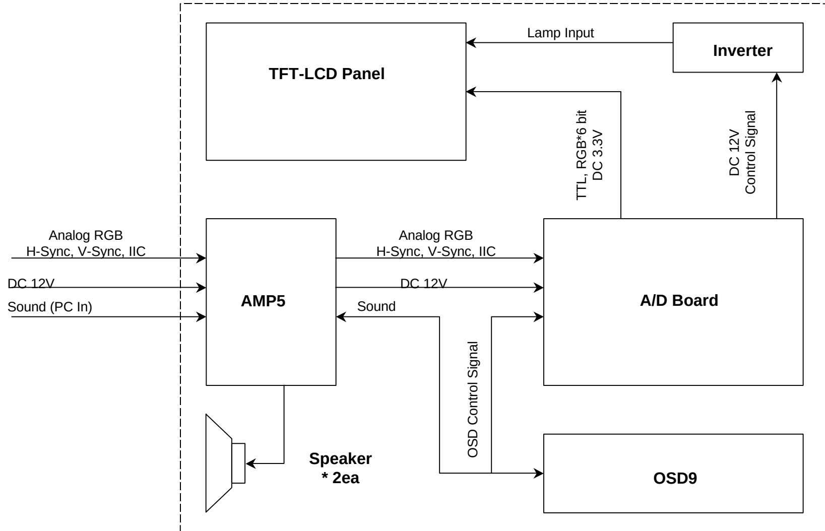
NLM155A1 LCD Monitor Block Diagram
