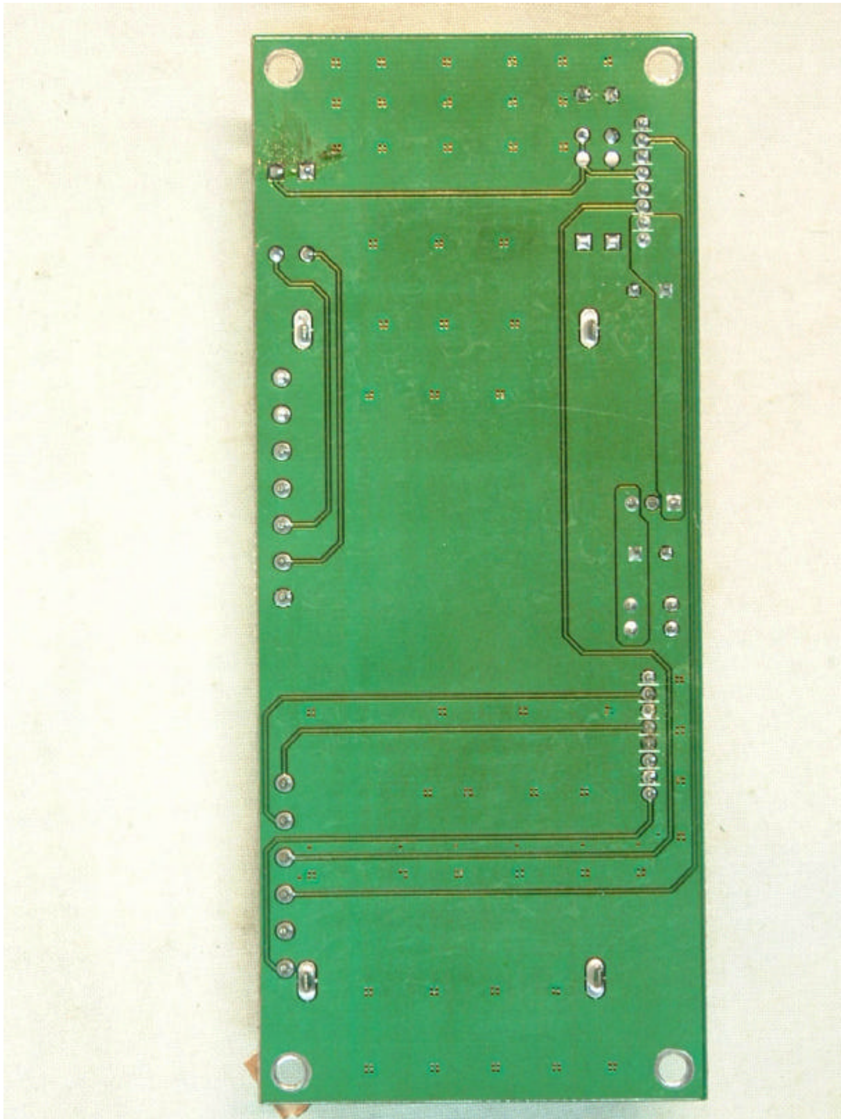
<REAR VIEW OF ZTR5A BOARD >
