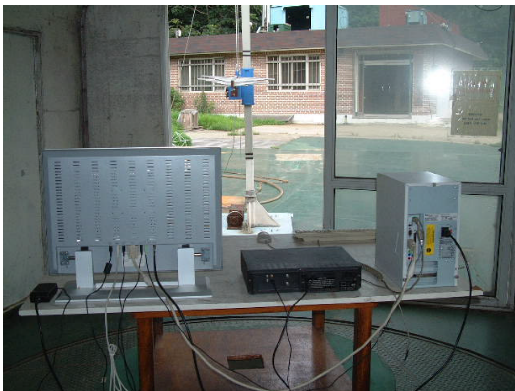
RADIATED EMISSION SETUP PHOTOGRAPH - REAR VIEW ( 300 - 1000 MHz )
