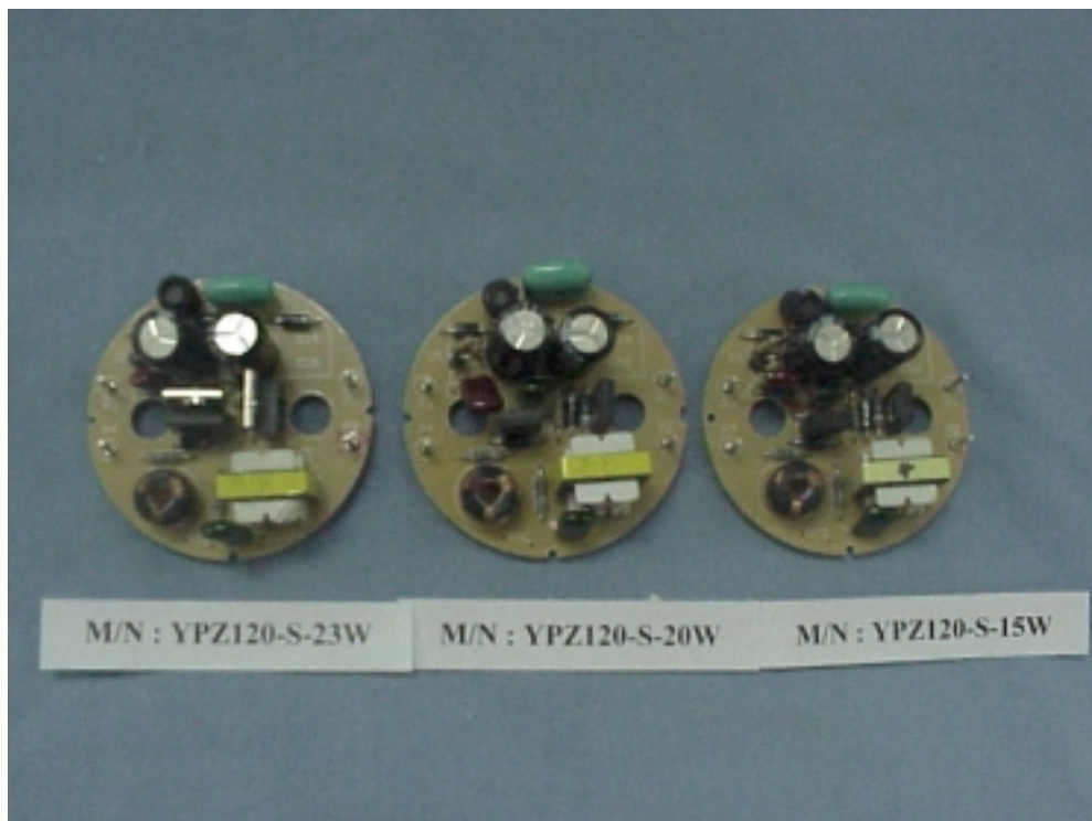
Figure 5 Energy Saving Lamp (M/N: YPZ120-S Series) Main Board (Component Side)
