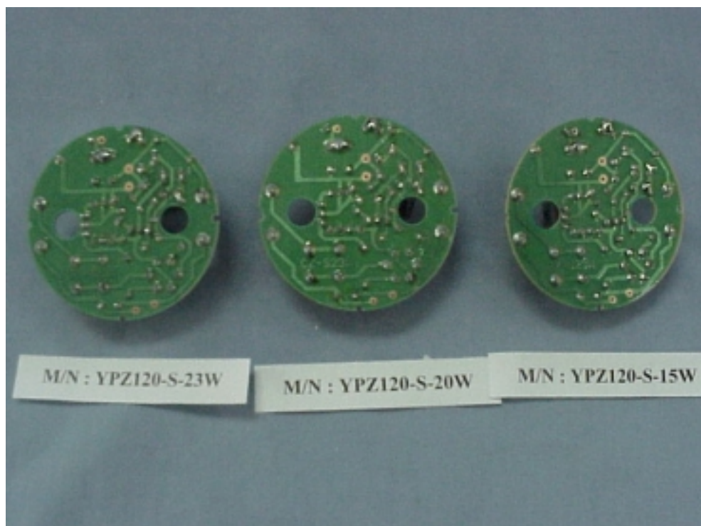
Figure 6 Energy Saving Lamp (M/N: YPZ120-S Series) Main Board (Soldered Side)
