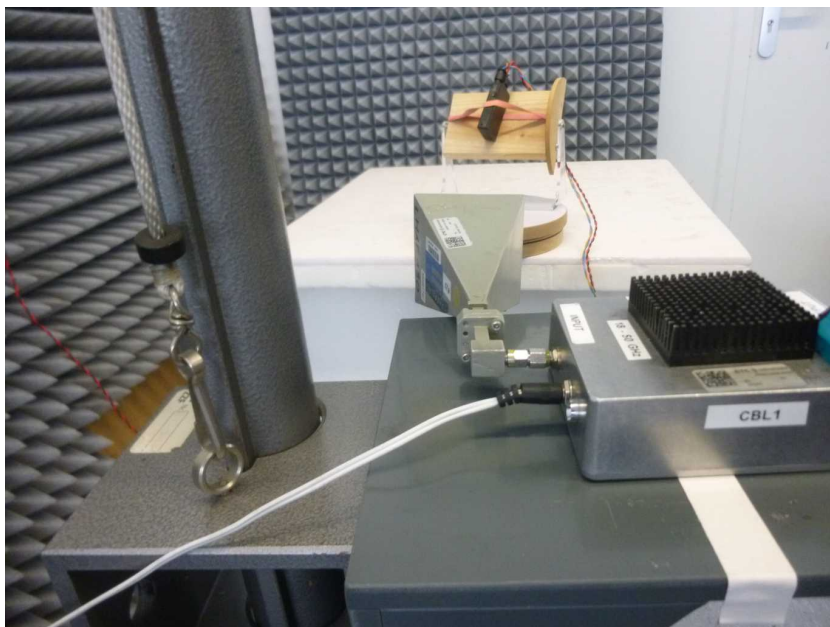
Photo 8: UWB 18 GHz to 40 GHz test setup
