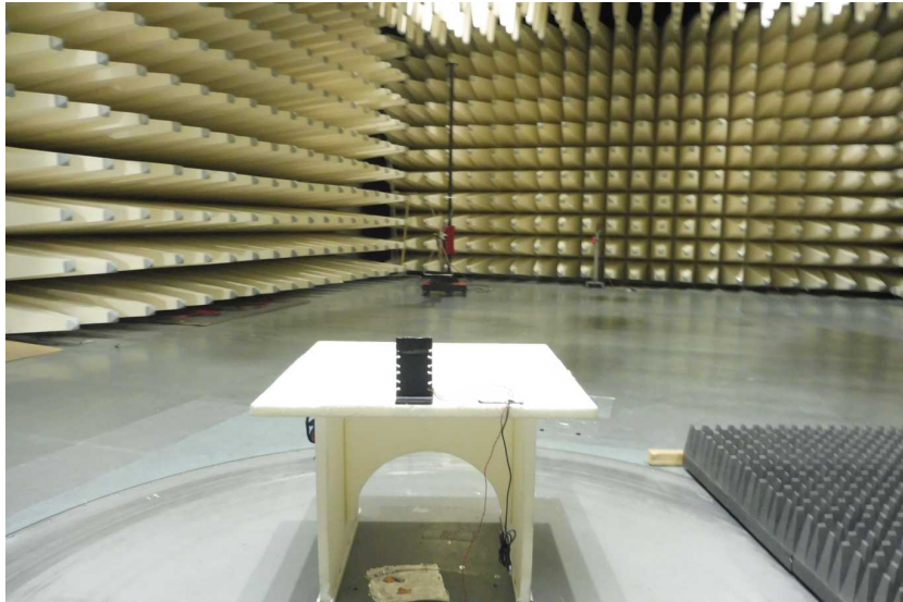
Photo 7: EUT at the semi-anechoic chamber, below 1 GHz test setup
