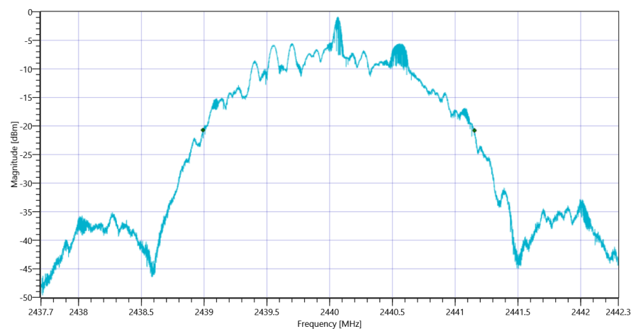
Plot_FCC Part 15.247 Bandwidth 99PCT-20dB ~ BT LE 2 Msps 20dB_27042021_104819.png
