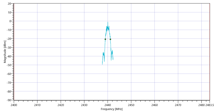
Plot_FCC Part 15.247 Bandwidth 99PCT-20dB ~ BT LE 2 Msps_27042021_104825.png
