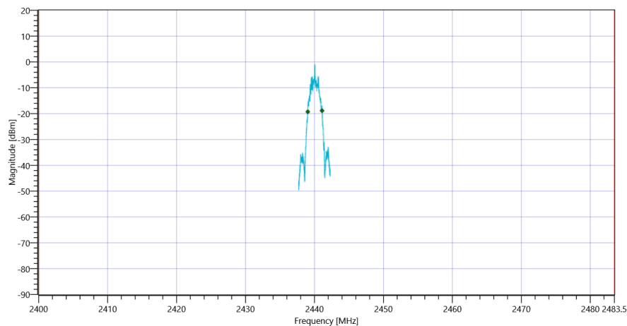
Plot_FCC Part 15.247 Bandwidth 99PCT-20dB ~ BT LE 2 Msps 99PCT_27042021_104811.png
