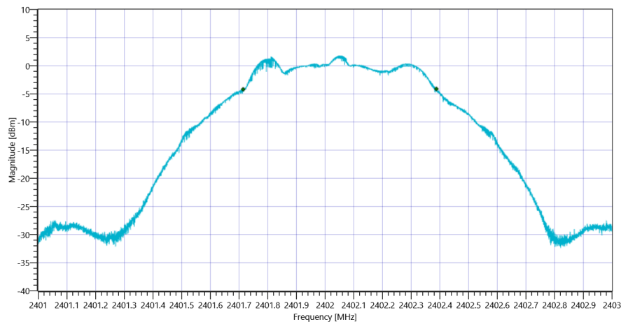
Plot_FCC Part 15.247 Maximum Peak Conducted Output Power DTS ~ BT LE coded S2 DTS BW_27042021_111235.png
