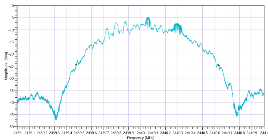
Plot_FCC Part 15.247 Bandwidth 99PCT-20dB ~ BT LE 1 Msps 20dB_27042021_102110.png
