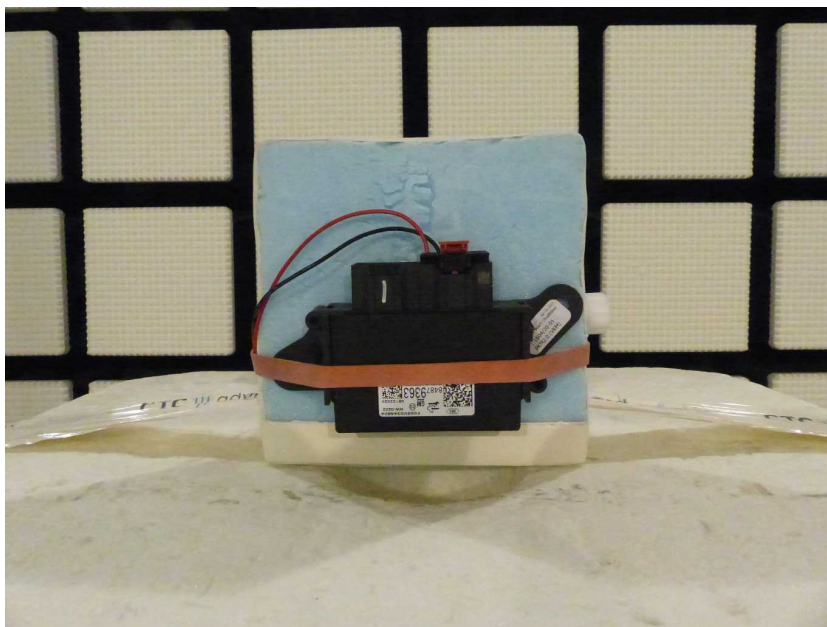
Photo 2: EUT at the fully anechoic chamber
