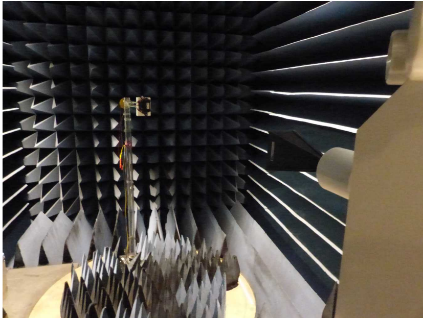
Photo 9: EUT at the anechoic chamber (10-18 GHz)
