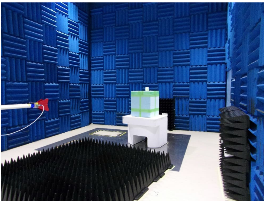
Above 1GHz
