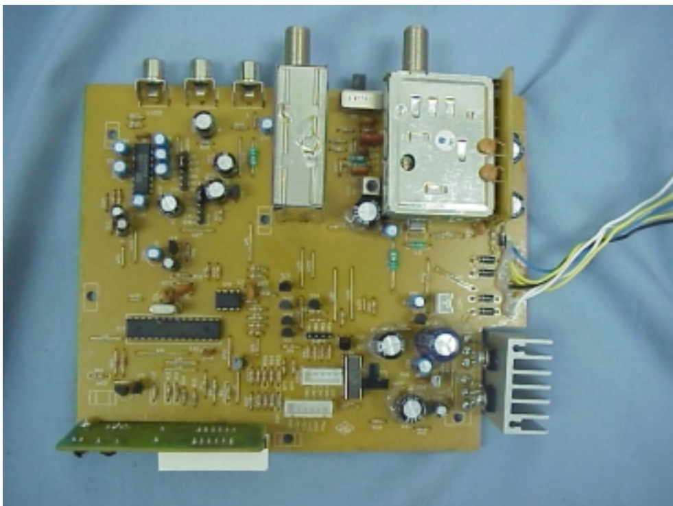
Figure 2 Remote Control Cable Converter (M/N: F3388U) MAIN BOARD (COMPONENT SIDE)
