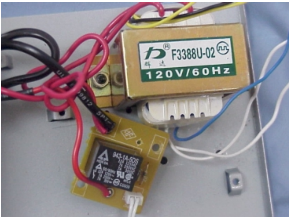
Figure 4 Remote Control Cable Converter (M/N: F3388U) POWER BOARD (COMPONENT SIDE)
