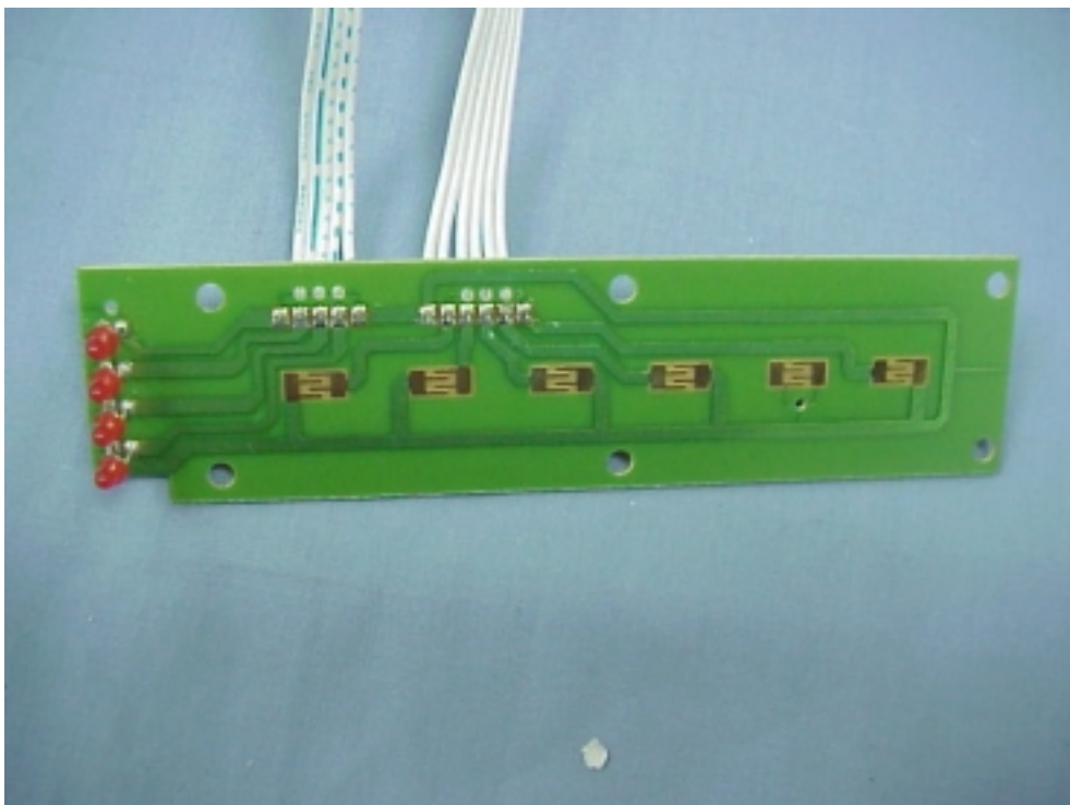
Figure 6 Remote Control Cable Converter (M/N: F3388U) SWITCH BOARD (FRONT SIDE)
