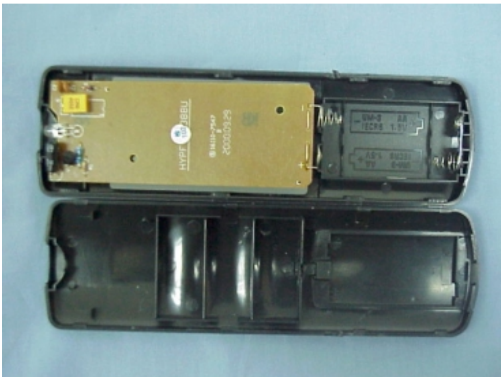
Figure 8 REMOTE CONTROL (COVER REMOVED) (Remote Control Cable Converter (M/N: F3388U))
