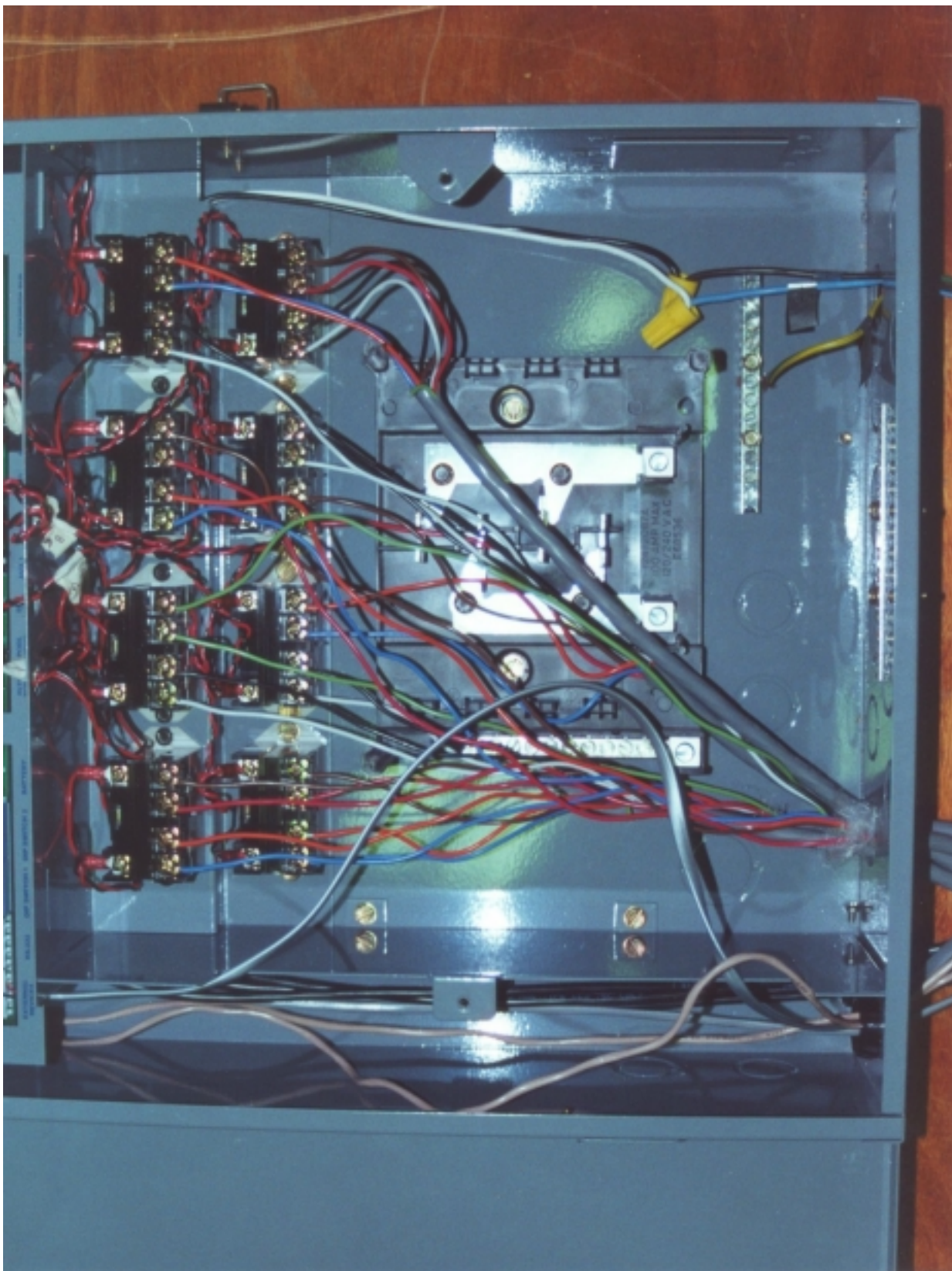
FRONT VIEW OF COMMAND CENTER (RELAYS)
