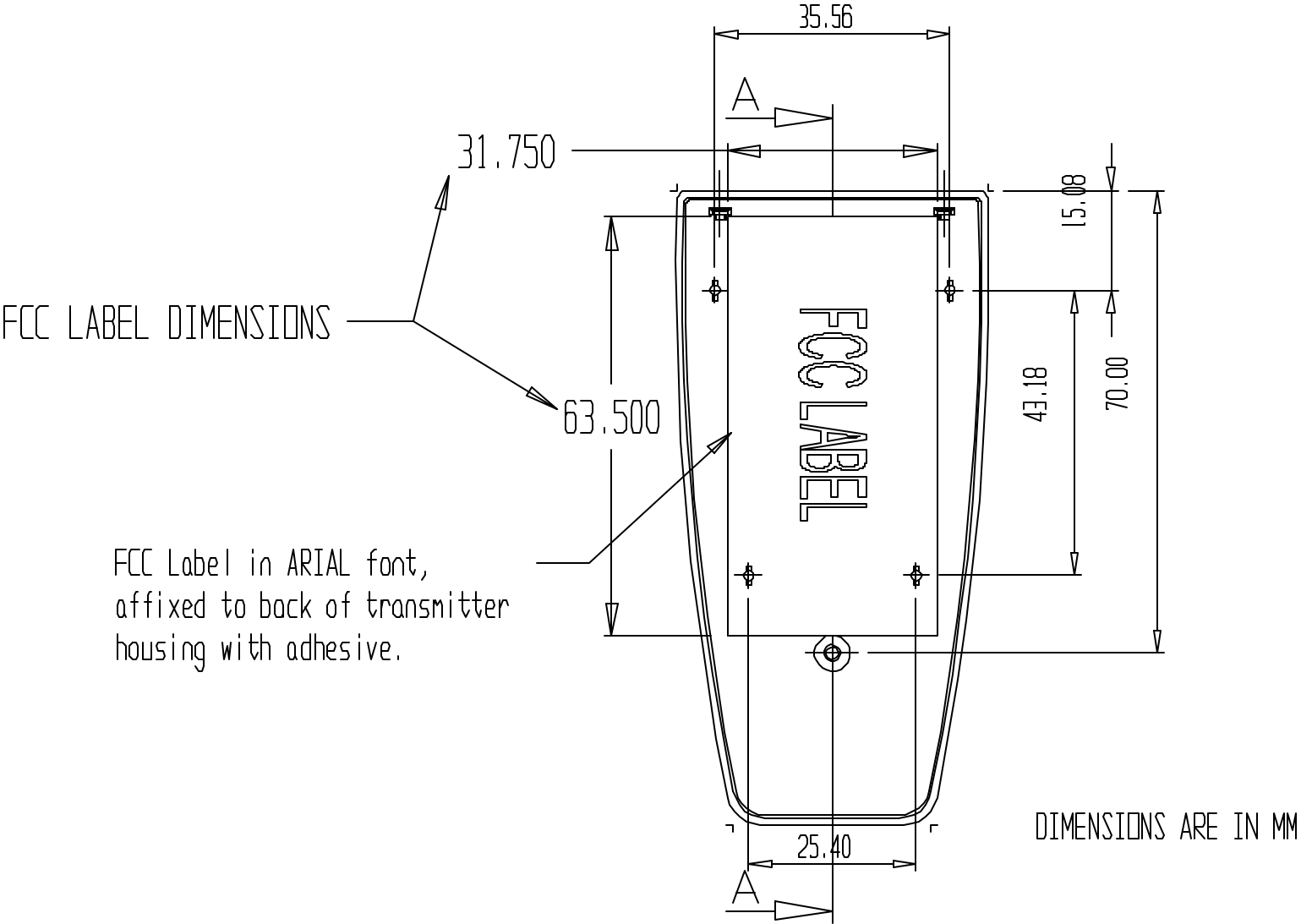
Bottom View of Transmitter
