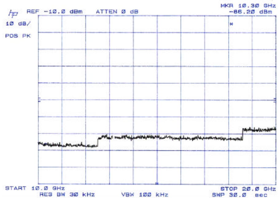
Spurious RF Conducted Emissions: 10.0GHz to 20.0GHz
